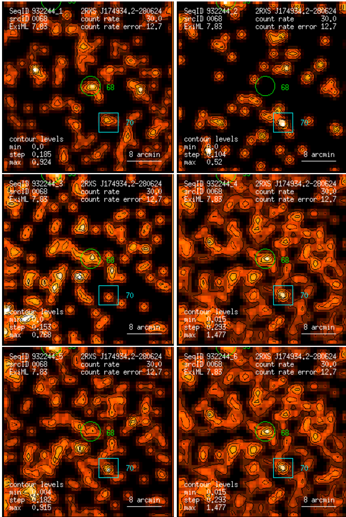
Figure 68: RASS 932244: detection 0068: band rate images, Gaussian filter: (1) PSPC channels 11 – 41, (2) 52 – 90, (3) 91 – 201, (4) 11 – 235, (5) 52 – 201, (6) 11 – 201. Broad band rates in counts/ks. Band rate contour levels in counts/ks/arcmin 2 .
