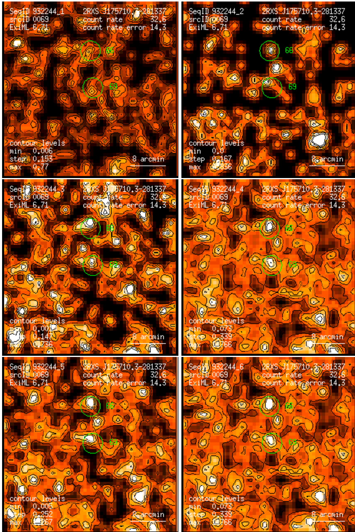
Figure 69: RASS 932244: detection 0069: band rate images, Gaussian filter: (1) PSPC channels 11 – 41, (2) 52 – 90, (3) 91 – 201, (4) 11 – 235, (5) 52 – 201, (6) 11 – 201. Broad band rates in counts/ks. Band rate contour levels in counts/ks/arcmin 2 .
