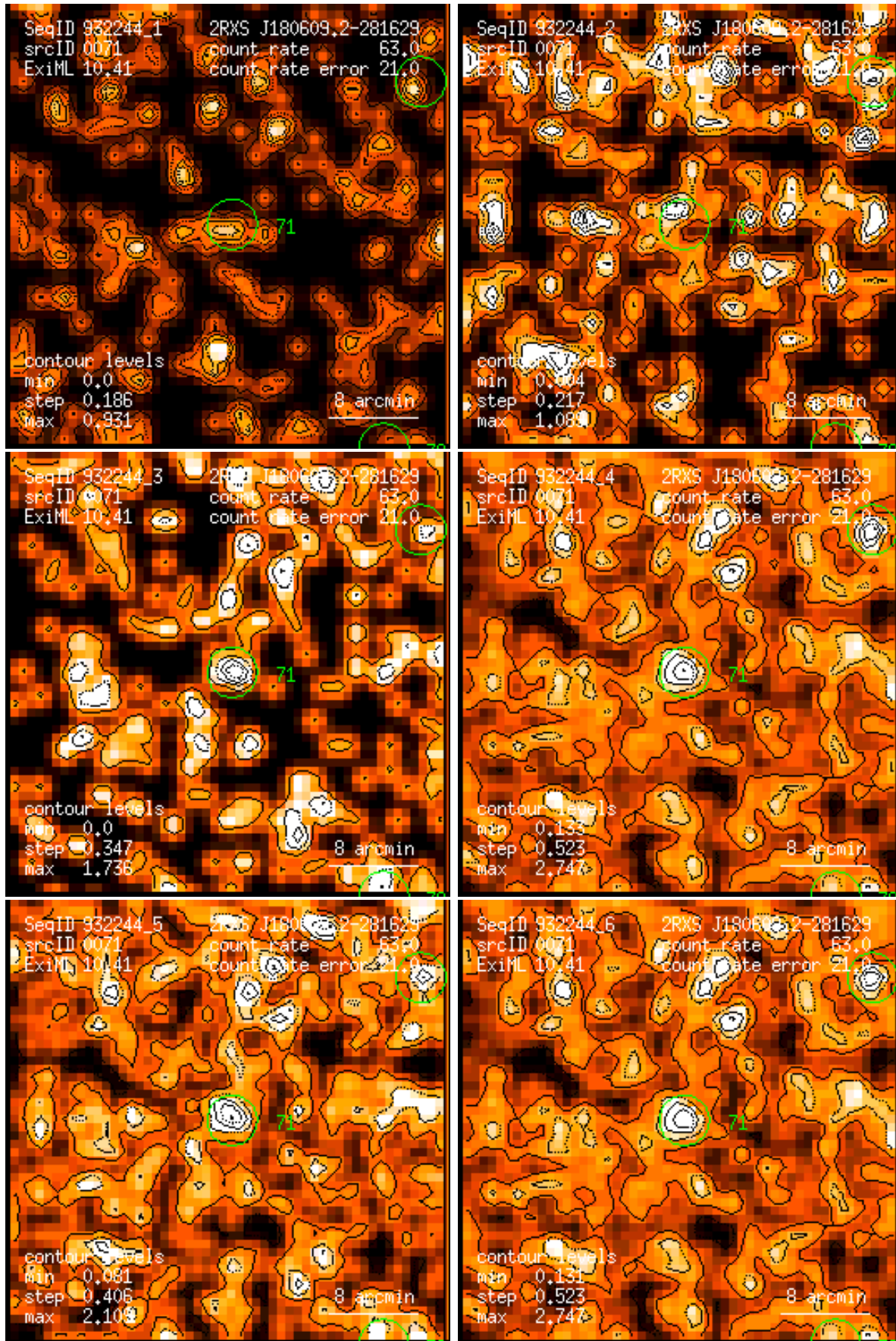
Figure 71: RASS 932244: detection 0071: band rate images, Gaussian filter: (1) PSPC channels 11 – 41, (2) 52 – 90, (3) 91 – 201, (4) 11 – 235, (5) 52 – 201, (6) 11 – 201. Broad band rates in counts/ks. Band rate contour levels in counts/ks/arcmin 2 .
