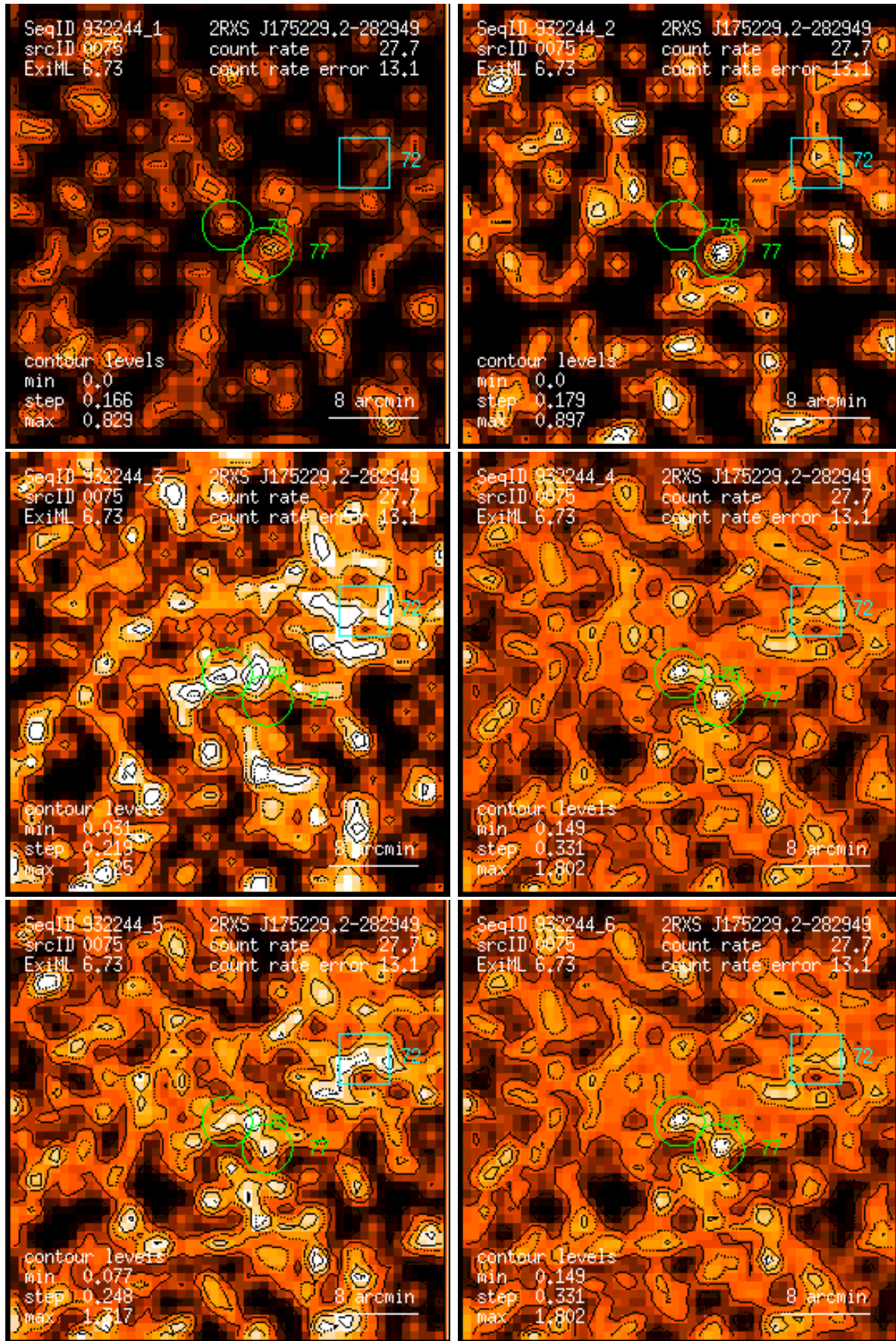
Figure 75: RASS 932244: detection 0075: band rate images, Gaussian filter: (1) PSPC channels 11 – 41, (2) 52 – 90, (3) 91 – 201, (4) 11 – 235, (5) 52 – 201, (6) 11 – 201. Broad band rates in counts/ks. Band rate contour levels in counts/ks/arcmin 2 .
