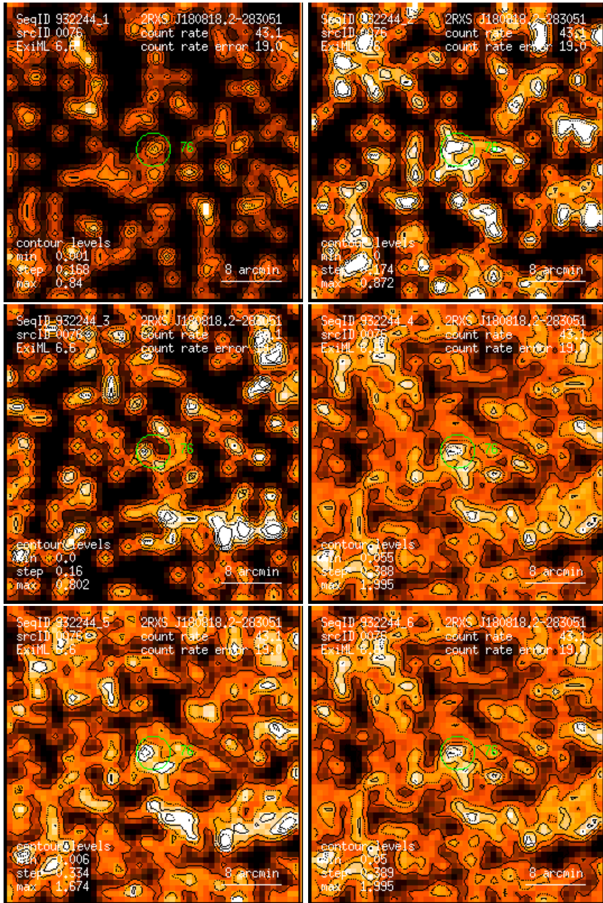
Figure 76: RASS 932244: detection 0076: band rate images, Gaussian filter: (1) PSPC channels 11 – 41, (2) 52 – 90, (3) 91 – 201, (4) 11 – 235, (5) 52 – 201, (6) 11 – 201. Broad band rates in counts/ks. Band rate contour levels in counts/ks/arcmin 2 .
