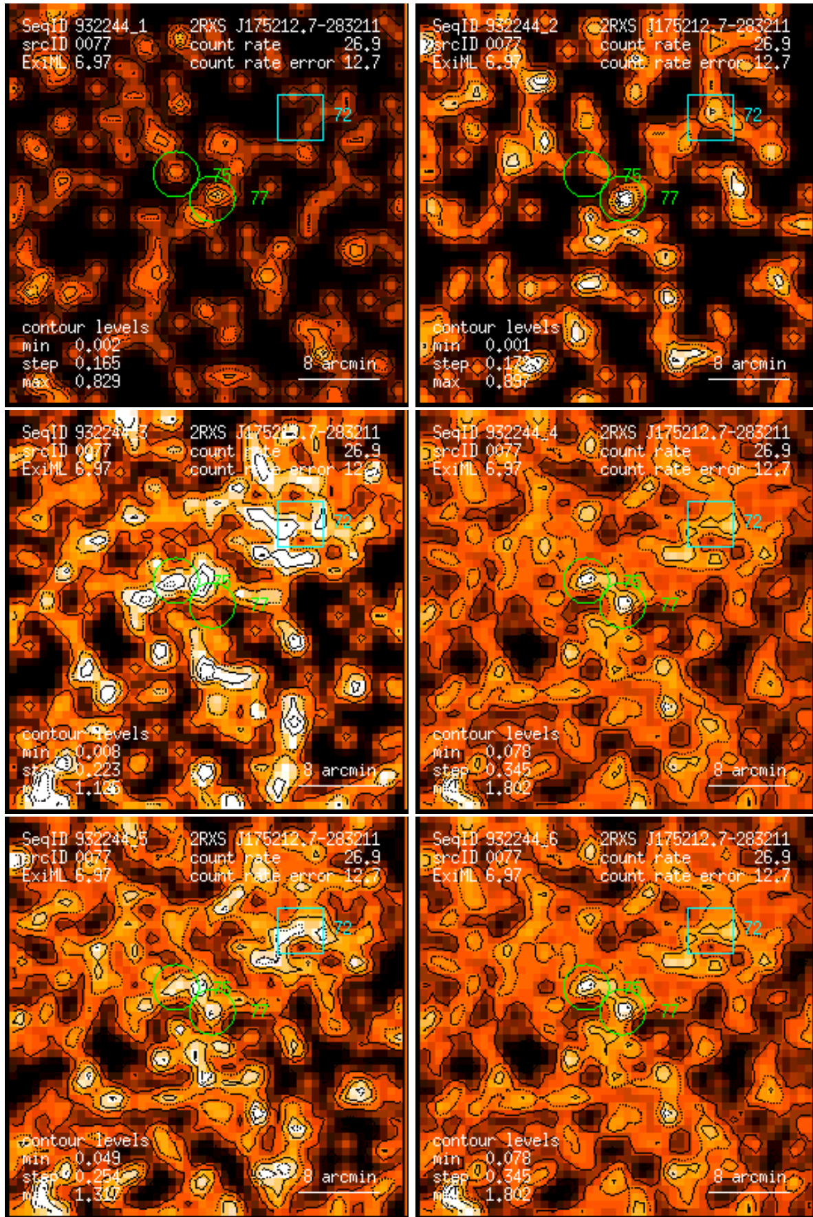
Figure 77: RASS 932244: detection 0077: band rate images, Gaussian filter: (1) PSPC channels 11 – 41, (2) 52 – 90, (3) 91 – 201, (4) 11 – 235, (5) 52 – 201, (6) 11 – 201. Broad band rates in counts/ks. Band rate contour levels in counts/ks/arcmin 2 .
