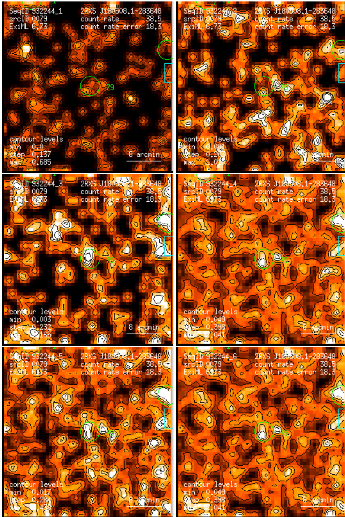
Figure 79: RASS 932244: detection 0079: band rate images, Gaussian filter: (1) PSPC channels 11 – 41, (2) 52 – 90, (3) 91 – 201, (4) 11 – 235, (5) 52 – 201, (6) 11 – 201. Broad band rates in counts/ks. Band rate contour levels in counts/ks/arcmin 2 .
