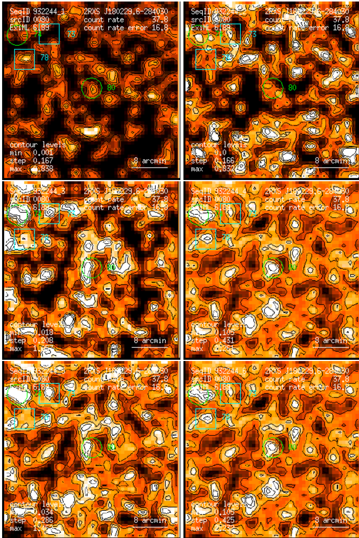
Figure 80: RASS 932244: detection 0080: band rate images, Gaussian filter: (1) PSPC channels 11 – 41, (2) 52 – 90, (3) 91 – 201, (4) 11 – 235, (5) 52 – 201, (6) 11 – 201. Broad band rates in counts/ks. Band rate contour levels in counts/ks/arcmin 2 .
