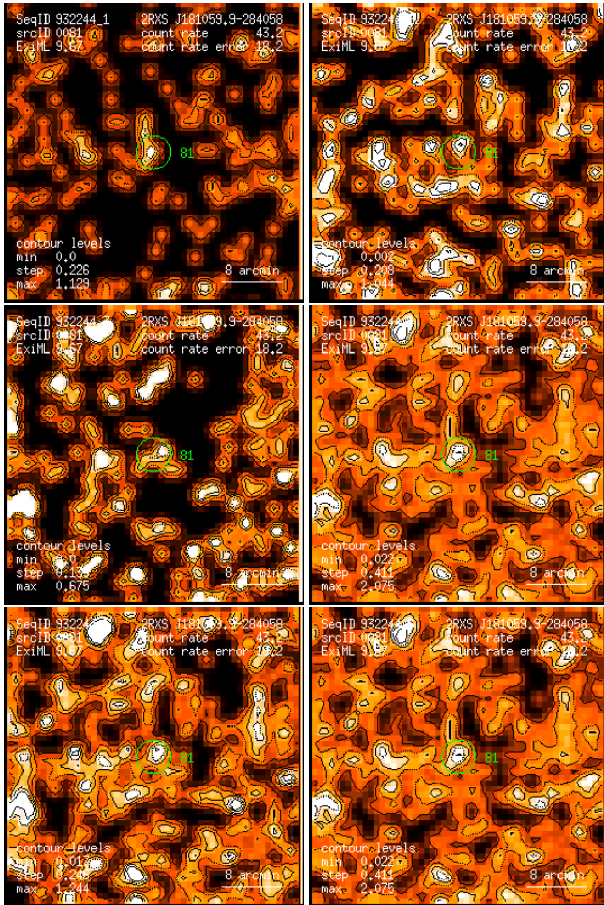
Figure 81: RASS 932244: detection 0081: band rate images, Gaussian filter: (1) PSPC channels 11 – 41, (2) 52 – 90, (3) 91 – 201, (4) 11 – 235, (5) 52 – 201, (6) 11 – 201. Broad band rates in counts/ks. Band rate contour levels in counts/ks/arcmin 2 .
