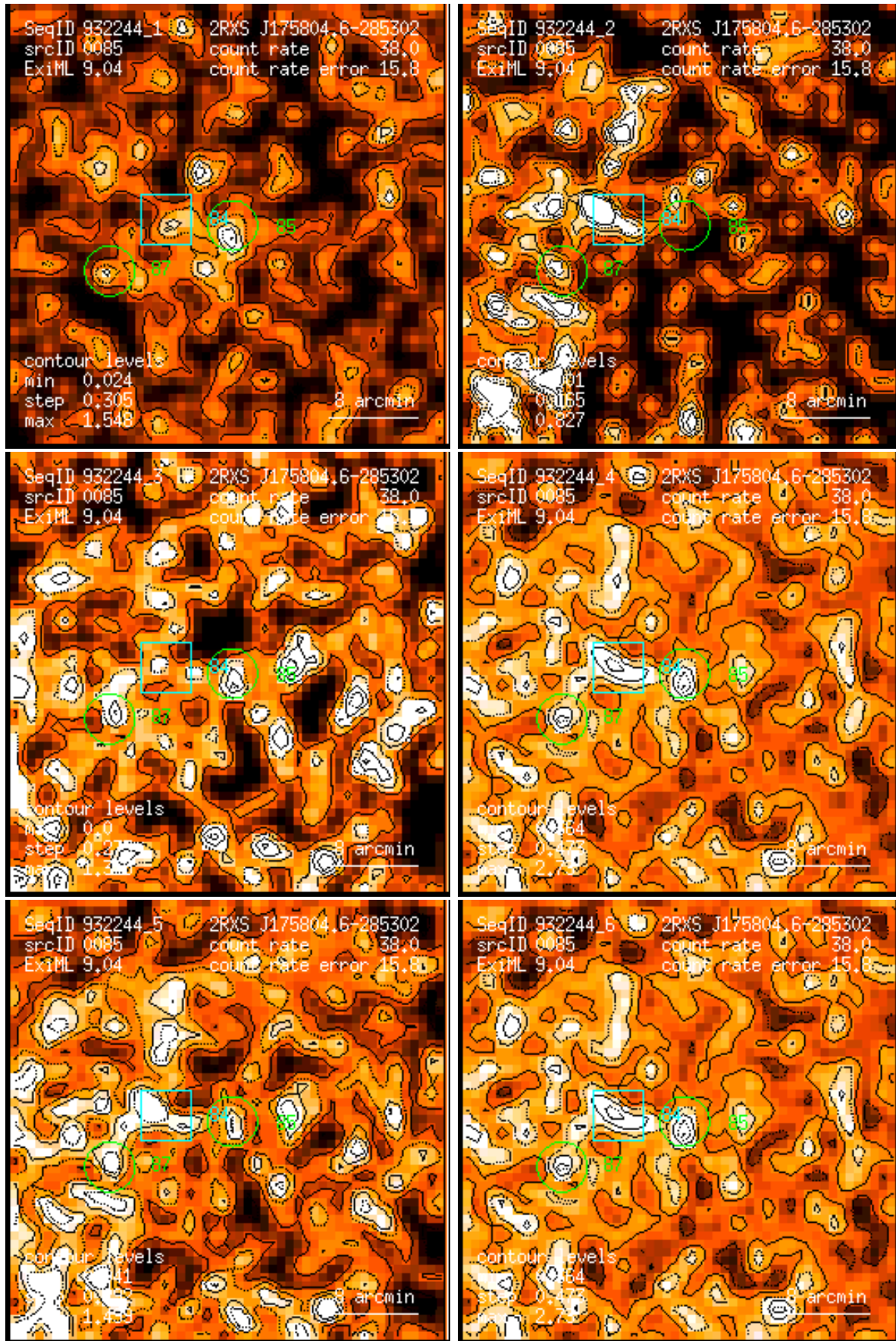
Figure 85: RASS 932244: detection 0085: band rate images, Gaussian filter: (1) PSPC channels 11 – 41, (2) 52 – 90, (3) 91 – 201, (4) 11 – 235, (5) 52 – 201, (6) 11 – 201. Broad band rates in counts/ks. Band rate contour levels in counts/ks/arcmin 2 .
