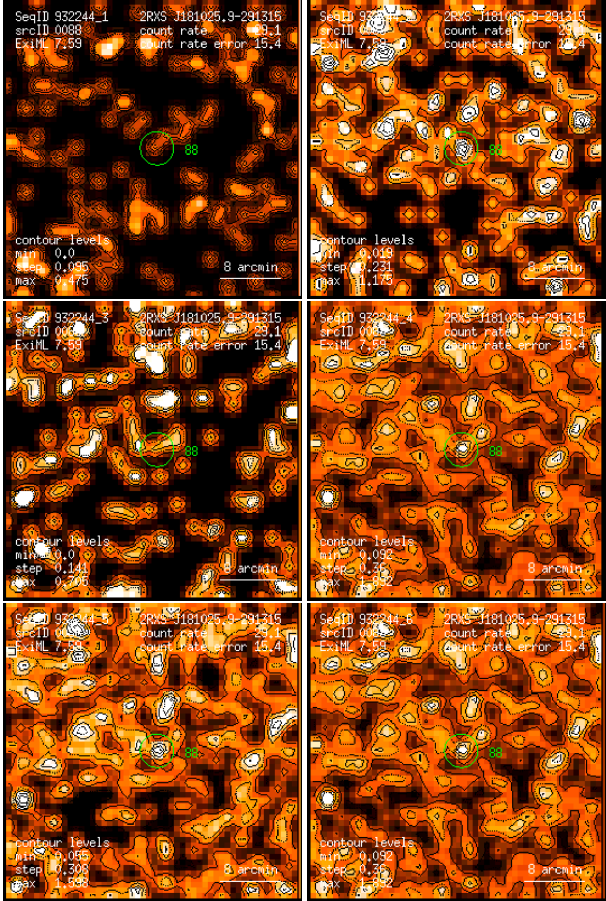
Figure 88: RASS 932244: detection 0088: band rate images, Gaussian filter: (1) PSPC channels 11 – 41, (2) 52 – 90, (3) 91 – 201, (4) 11 – 235, (5) 52 – 201, (6) 11 – 201. Broad band rates in counts/ks. Band rate contour levels in counts/ks/arcmin 2 .
