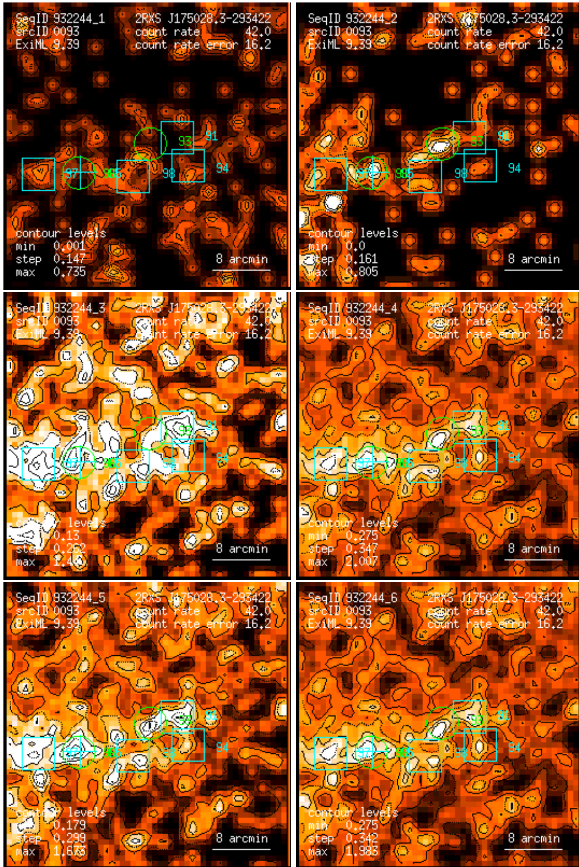
Figure 93: RASS 932244: detection 0093: band rate images, Gaussian filter: (1) PSPC channels 11 – 41, (2) 52 – 90, (3) 91 – 201, (4) 11 – 235, (5) 52 – 201, (6) 11 – 201. Broad band rates in counts/ks. Band rate contour levels in counts/ks/arcmin 2 .
