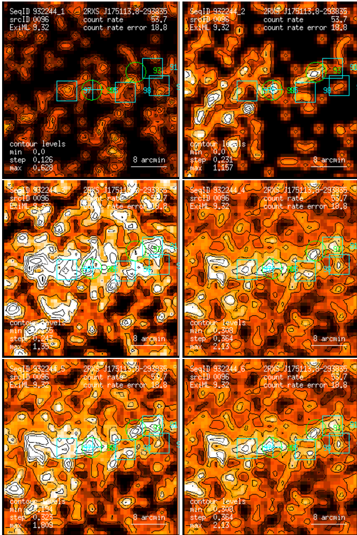
Figure 96: RASS 932244: detection 0096: band rate images, Gaussian filter: (1) PSPC channels 11 – 41, (2) 52 – 90, (3) 91 – 201, (4) 11 – 235, (5) 52 – 201, (6) 11 – 201. Broad band rates in counts/ks. Band rate contour levels in counts/ks/arcmin 2 .
