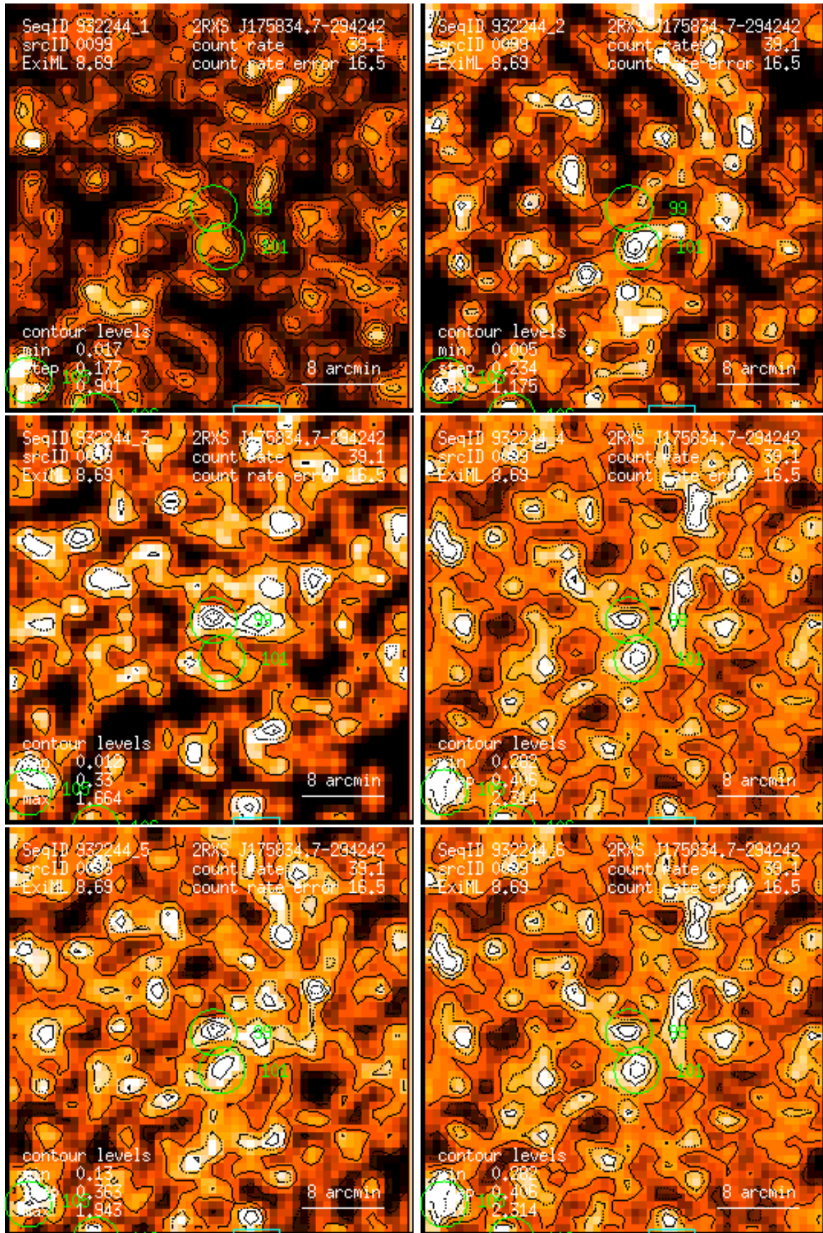
Figure 99: RASS 932244: detection 0099: band rate images, Gaussian filter: (1) PSPC channels 11 – 41, (2) 52 – 90, (3) 91 – 201, (4) 11 – 235, (5) 52 – 201, (6) 11 – 201. Broad band rates in counts/ks. Band rate contour levels in counts/ks/arcmin 2 .
