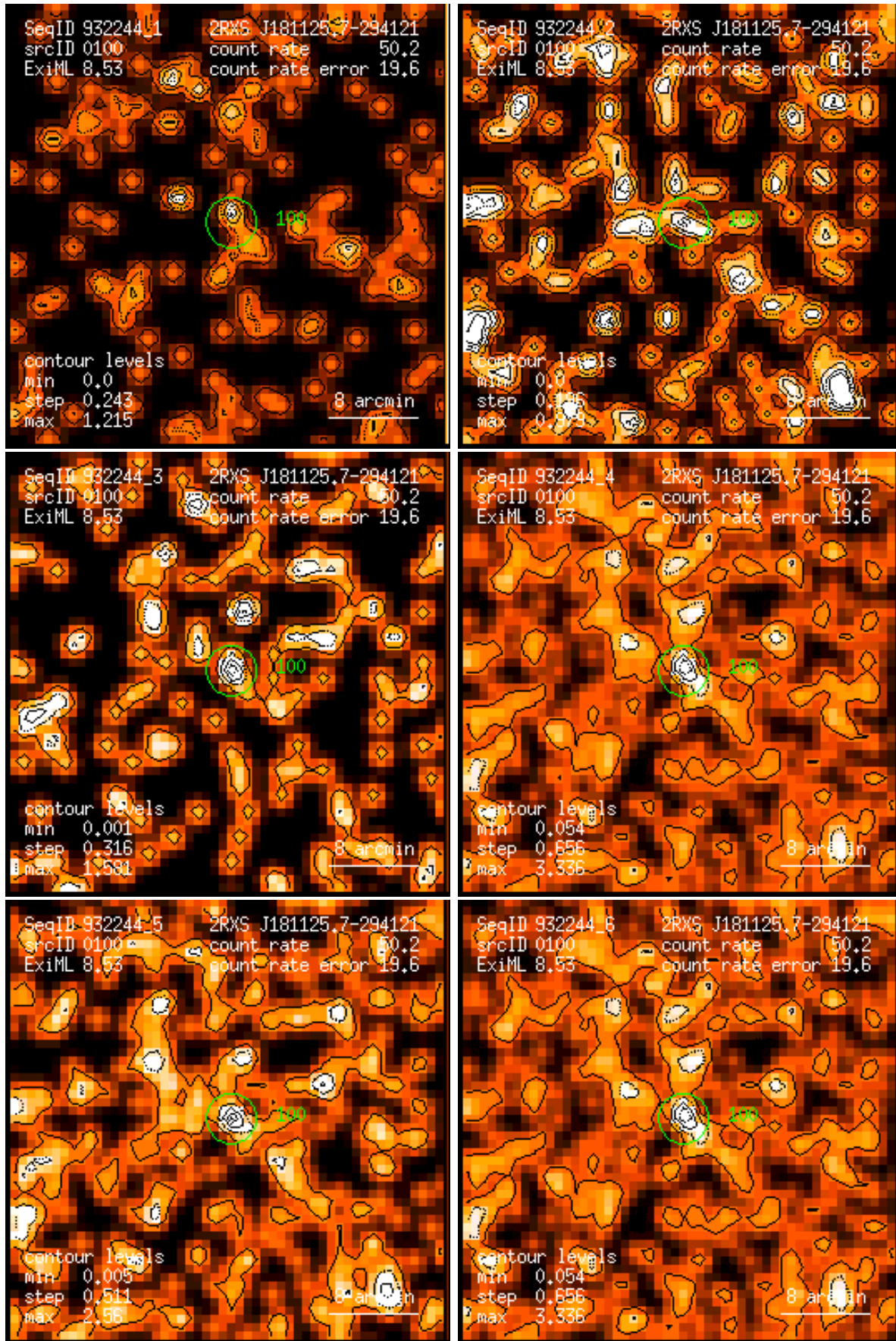
Figure 100: RASS 932244: detection 0100: band rate images, Gaussian filter: (1) PSPC channels 11 – 41, (2) 52 – 90, (3) 91 – 201, (4) 11 – 235, (5) 52 – 201, (6) 11 – 201. Broad band rates in counts/ks. Band rate contour levels in counts/ks/arcmin 2 .
