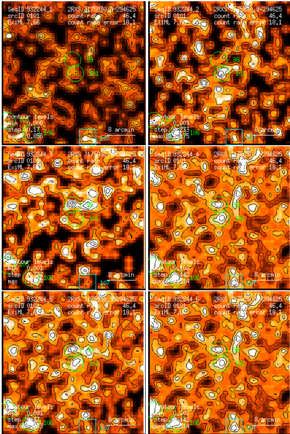
Figure 101: RASS 932244: detection 0101: band rate images, Gaussian filter: (1) PSPC channels 11 – 41, (2) 52 – 90, (3) 91 – 201, (4) 11 – 235, (5) 52 – 201, (6) 11 – 201. Broad band rates in counts/ks. Band rate contour levels in counts/ks/arcmin 2 .
