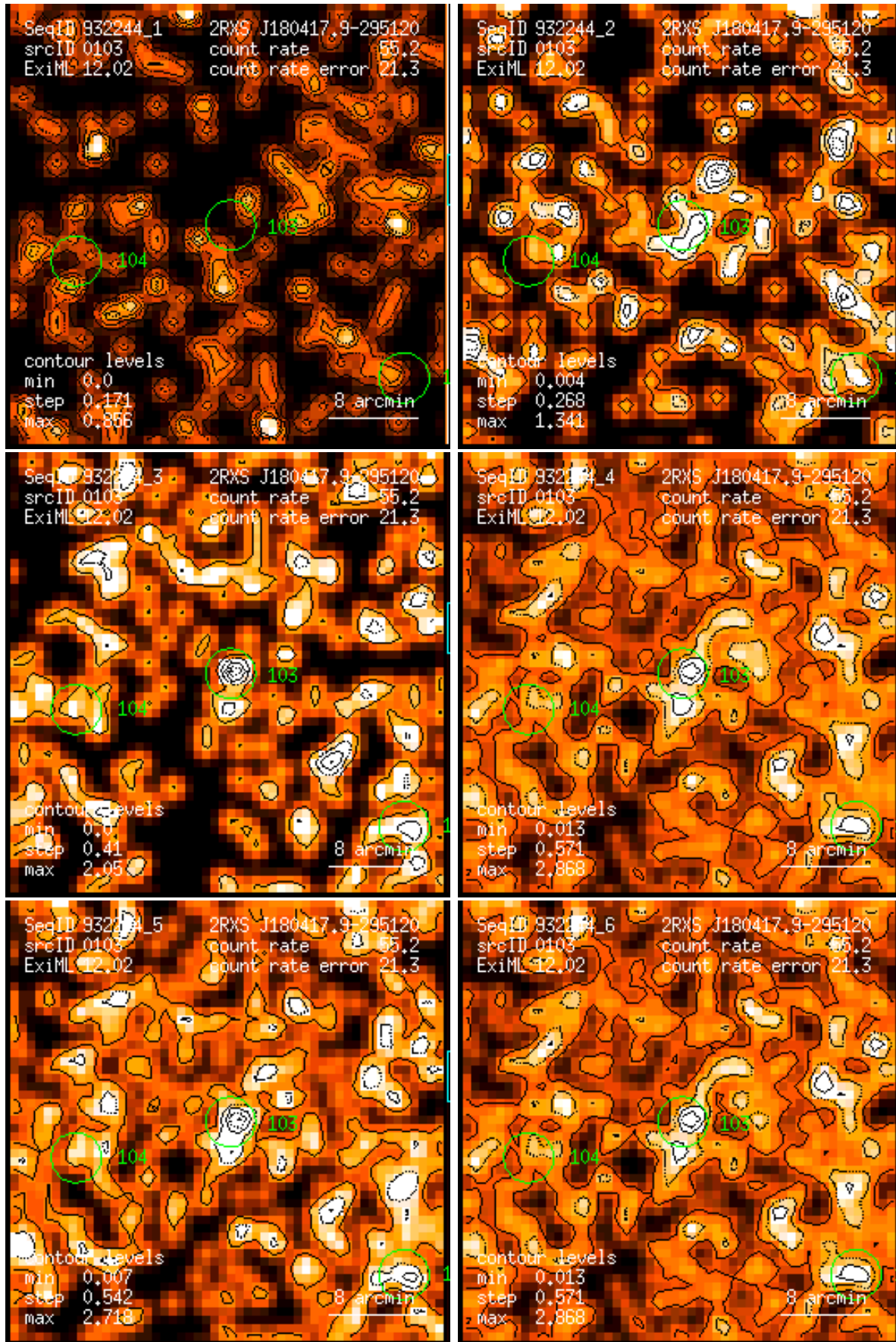
Figure 103: RASS 932244: detection 0103: band rate images, Gaussian filter: (1) PSPC channels 11 – 41, (2) 52 – 90, (3) 91 – 201, (4) 11 – 235, (5) 52 – 201, (6) 11 – 201. Broad band rates in counts/ks. Band rate contour levels in counts/ks/arcmin 2 .
