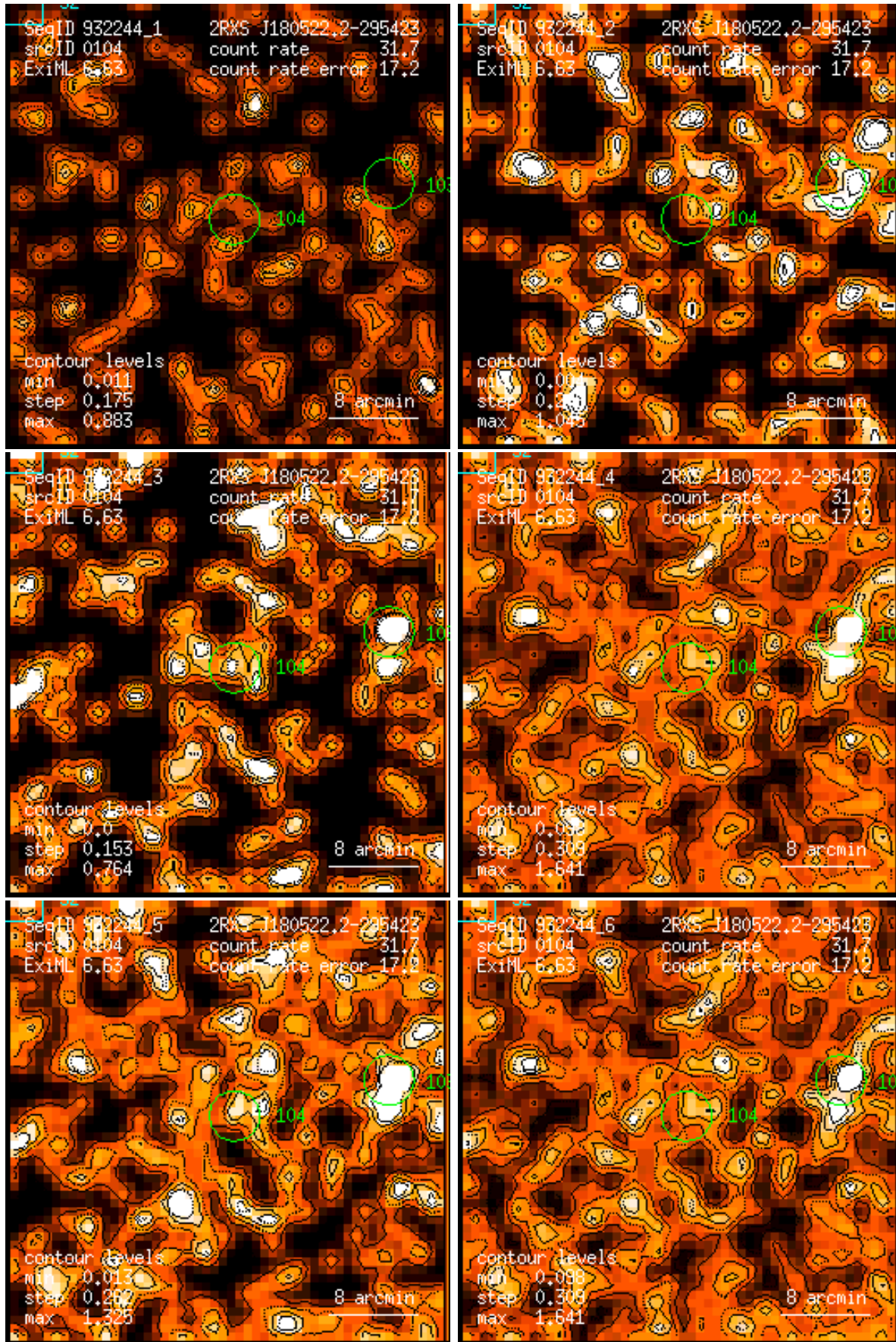
Figure 104: RASS 932244: detection 0104: band rate images, Gaussian filter: (1) PSPC channels 11 – 41, (2) 52 – 90, (3) 91 – 201, (4) 11 – 235, (5) 52 – 201, (6) 11 – 201. Broad band rates in counts/ks. Band rate contour levels in counts/ks/arcmin 2 .
