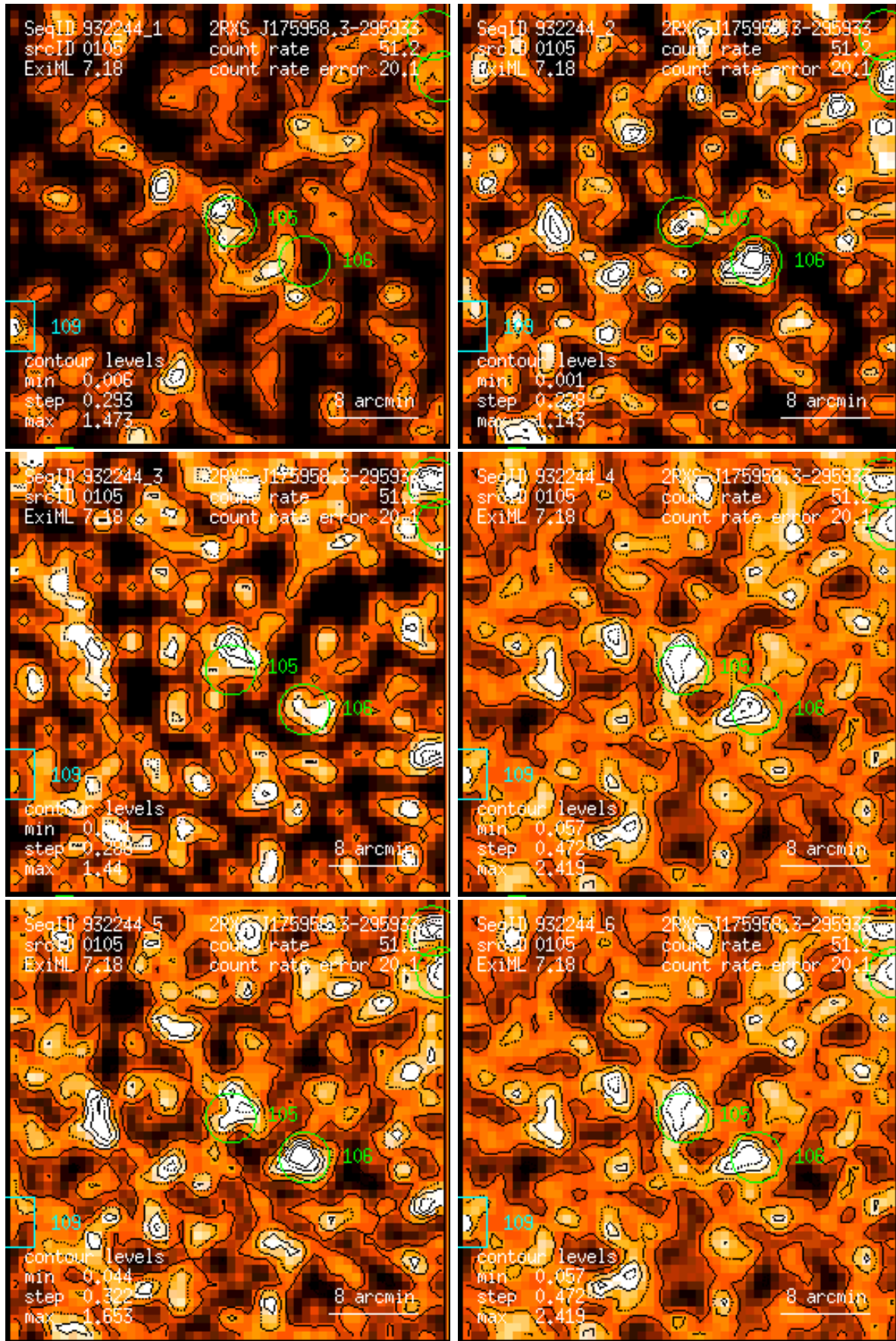
Figure 105: RASS 932244: detection 0105: band rate images, Gaussian filter: (1) PSPC channels 11 – 41, (2) 52 – 90, (3) 91 – 201, (4) 11 – 235, (5) 52 – 201, (6) 11 – 201. Broad band rates in counts/ks. Band rate contour levels in counts/ks/arcmin 2 .
