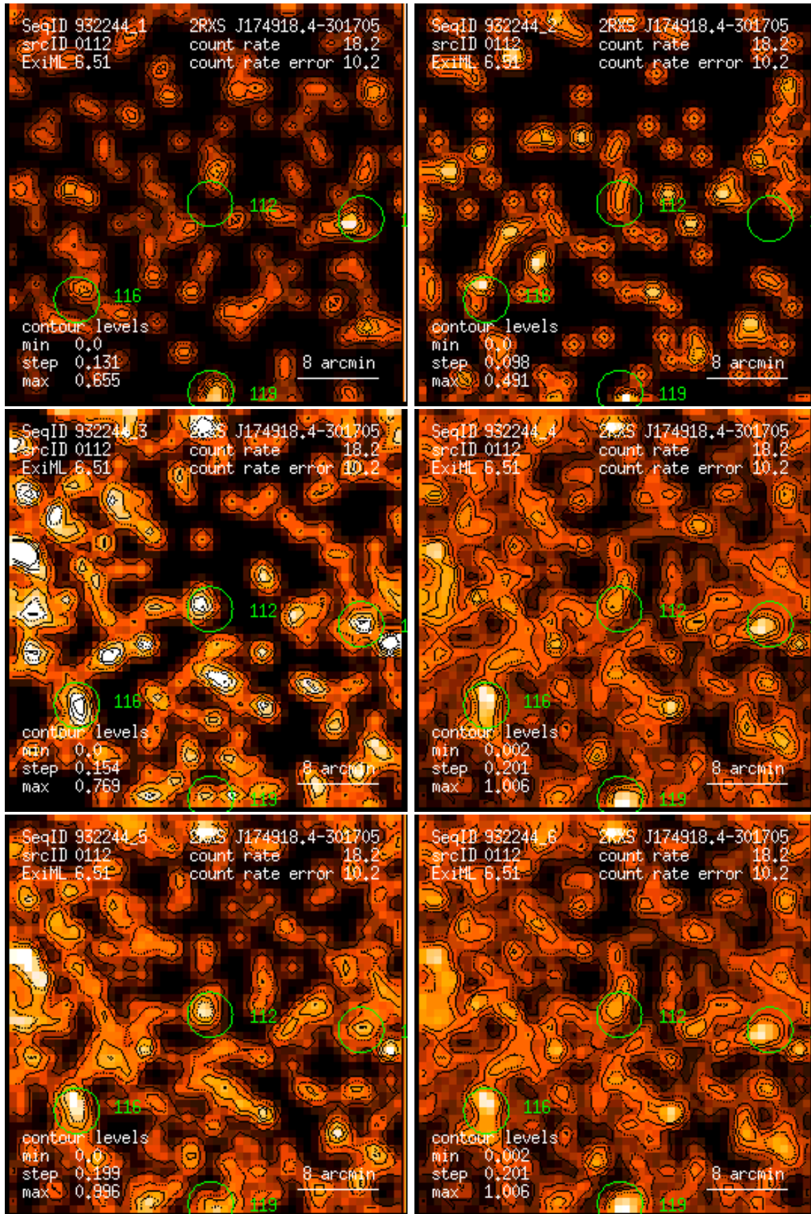
Figure 112: RASS 932244: detection 0112: band rate images, Gaussian filter: (1) PSPC channels 11 – 41, (2) 52 – 90, (3) 91 – 201, (4) 11 – 235, (5) 52 – 201, (6) 11 – 201. Broad band rates in counts/ks. Band rate contour levels in counts/ks/arcmin 2 .
