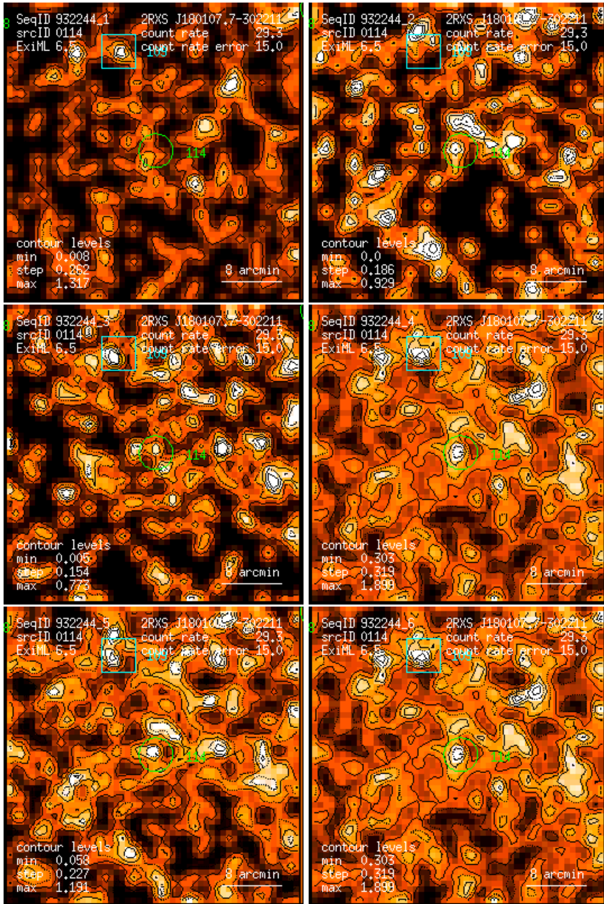
Figure 114: RASS 932244: detection 0114: band rate images, Gaussian filter: (1) PSPC channels 11 – 41, (2) 52 – 90, (3) 91 – 201, (4) 11 – 235, (5) 52 – 201, (6) 11 – 201. Broad band rates in counts/ks. Band rate contour levels in counts/ks/arcmin 2 .
