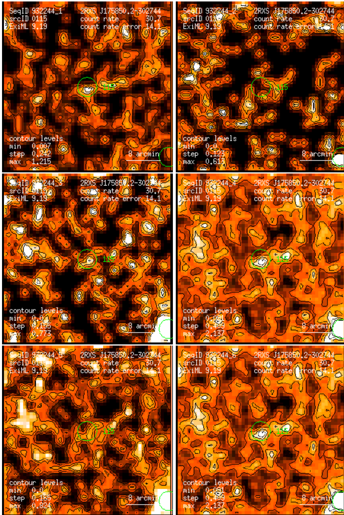
Figure 115: RASS 932244: detection 0115: band rate images, Gaussian filter: (1) PSPC channels 11 – 41, (2) 52 – 90, (3) 91 – 201, (4) 11 – 235, (5) 52 – 201, (6) 11 – 201. Broad band rates in counts/ks. Band rate contour levels in counts/ks/arcmin 2 .
