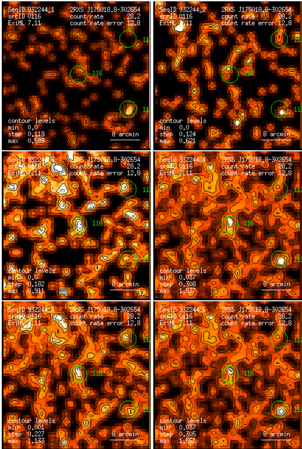
Figure 116: RASS 932244: detection 0116: band rate images, Gaussian filter: (1) PSPC channels 11 – 41, (2) 52 – 90, (3) 91 – 201, (4) 11 – 235, (5) 52 – 201, (6) 11 – 201. Broad band rates in counts/ks. Band rate contour levels in counts/ks/arcmin 2 .
