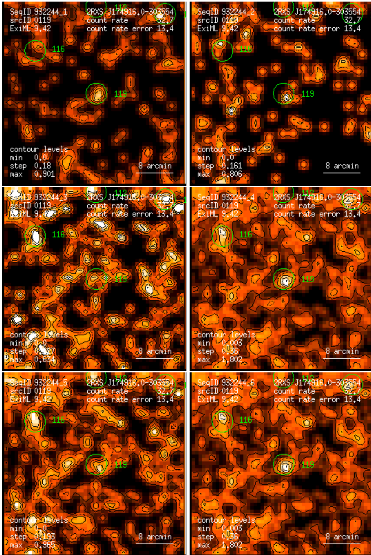
Figure 119: RASS 932244: detection 0119: band rate images, Gaussian filter: (1) PSPC channels 11 – 41, (2) 52 – 90, (3) 91 – 201, (4) 11 – 235, (5) 52 – 201, (6) 11 – 201. Broad band rates in counts/ks. Band rate contour levels in counts/ks/arcmin 2 .
