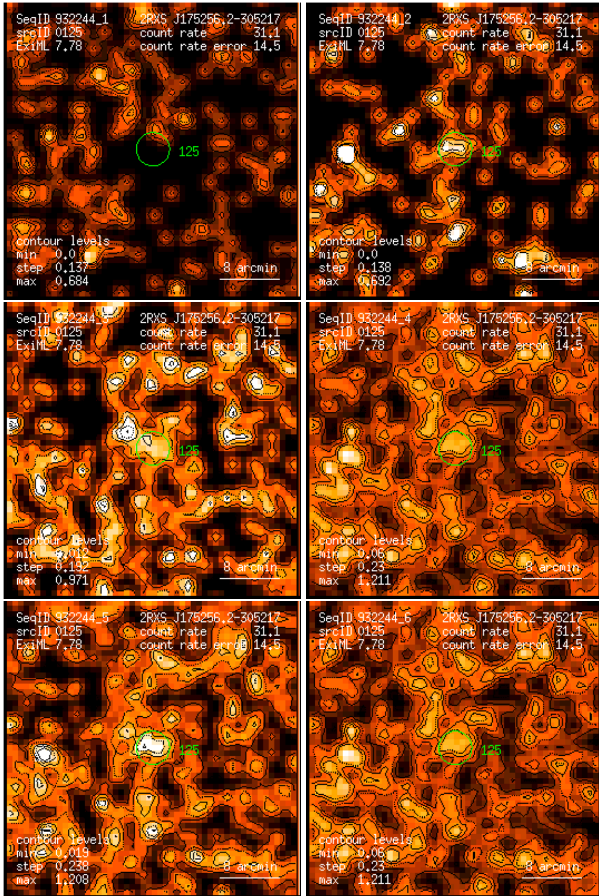
Figure 125: RASS 932244: detection 0125: band rate images, Gaussian filter: (1) PSPC channels 11 – 41, (2) 52 – 90, (3) 91 – 201, (4) 11 – 235, (5) 52 – 201, (6) 11 – 201. Broad band rates in counts/ks. Band rate contour levels in counts/ks/arcmin 2 .
