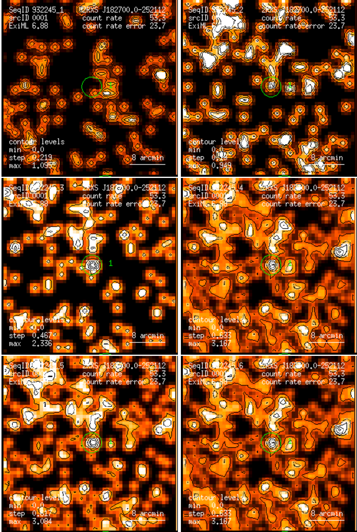
Figure 1: RASS 932245: detection 0001: band rate images, Gaussian filter: (1) PSPC channels 11 – 41, (2) 52 – 90, (3) 91 – 201, (4) 11 – 235, (5) 52 – 201, (6) 11 – 201. Broad band rates in counts/ks. Band rate contour levels in counts/ks/arcmin 2 .
