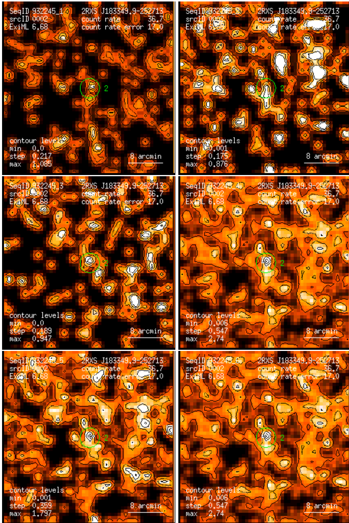
Figure 2: RASS 932245: detection 0002: band rate images, Gaussian filter: (1) PSPC channels 11 – 41, (2) 52 – 90, (3) 91 – 201, (4) 11 – 235, (5) 52 – 201, (6) 11 – 201. Broad band rates in counts/ks. Band rate contour levels in counts/ks/arcmin 2 .
