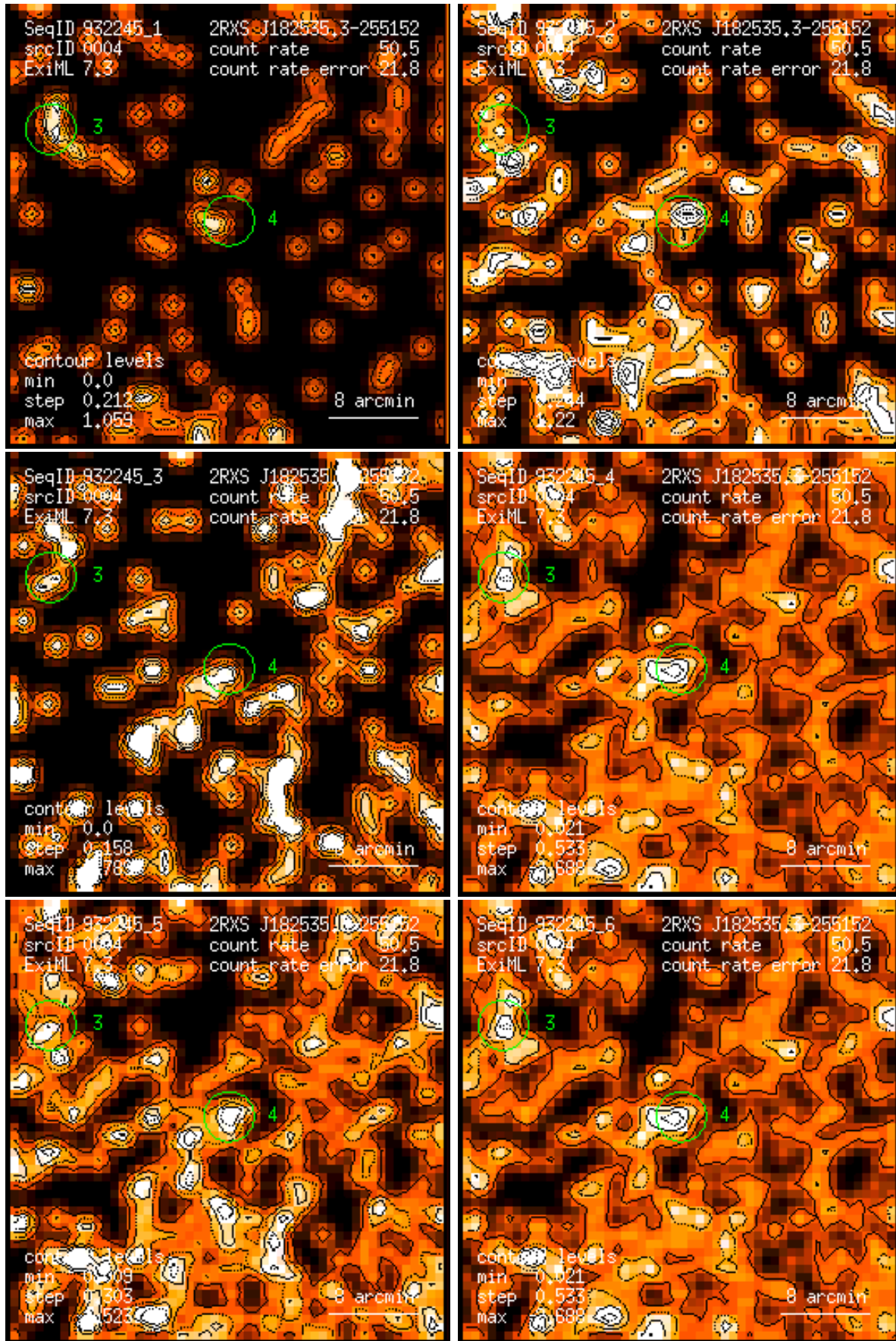
Figure 4: RASS 932245: detection 0004: band rate images, Gaussian filter: (1) PSPC channels 11 – 41, (2) 52 – 90, (3) 91 – 201, (4) 11 – 235, (5) 52 – 201, (6) 11 – 201. Broad band rates in counts/ks. Band rate contour levels in counts/ks/arcmin 2 .
