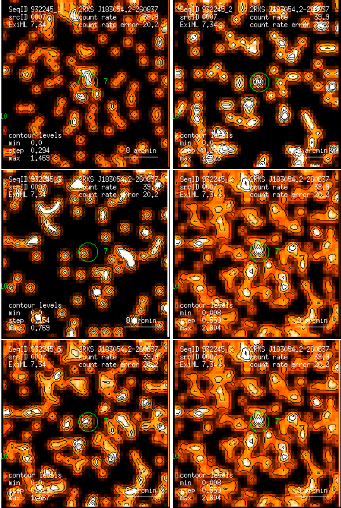
Figure 7: RASS 932245: detection 0007: band rate images, Gaussian filter: (1) PSPC channels 11 – 41, (2) 52 – 90, (3) 91 – 201, (4) 11 – 235, (5) 52 – 201, (6) 11 – 201. Broad band rates in counts/ks. Band rate contour levels in counts/ks/arcmin 2 .
