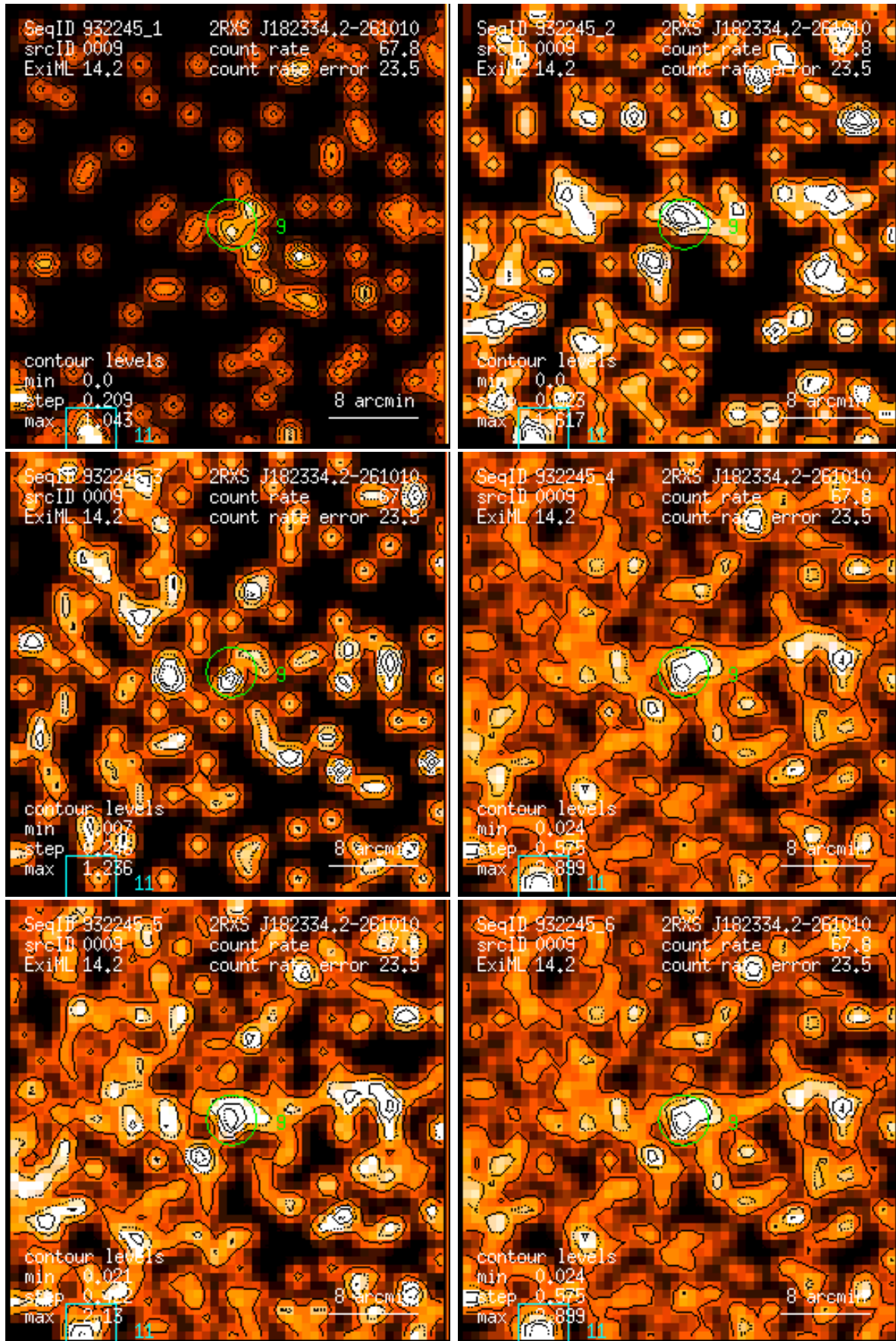
Figure 9: RASS 932245: detection 0009: band rate images, Gaussian filter: (1) PSPC channels 11 – 41, (2) 52 – 90, (3) 91 – 201, (4) 11 – 235, (5) 52 – 201, (6) 11 – 201. Broad band rates in counts/ks. Band rate contour levels in counts/ks/arcmin 2 .
