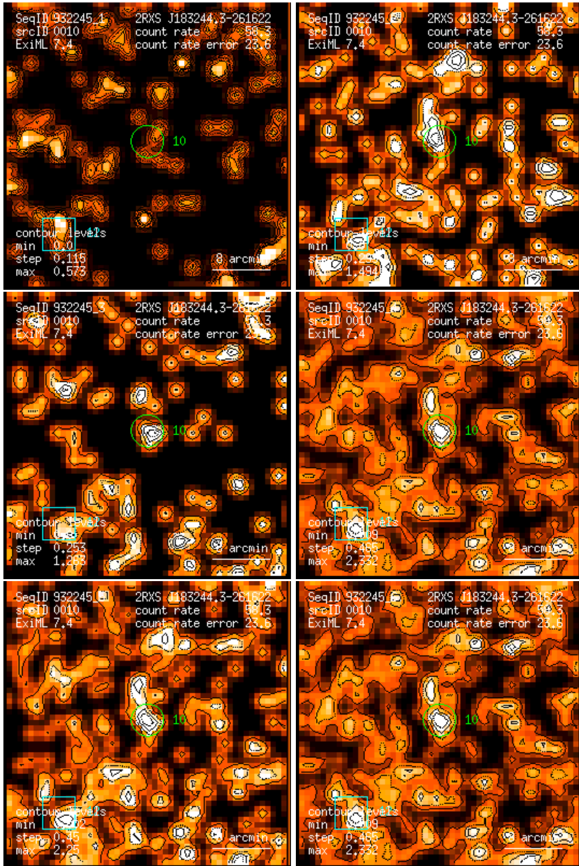
Figure 10: RASS 932245: detection 0010: band rate images, Gaussian filter: (1) PSPC channels 11 – 41, (2) 52 – 90, (3) 91 – 201, (4) 11 – 235, (5) 52 – 201, (6) 11 – 201. Broad band rates in counts/ks. Band rate contour levels in counts/ks/arcmin 2 .
