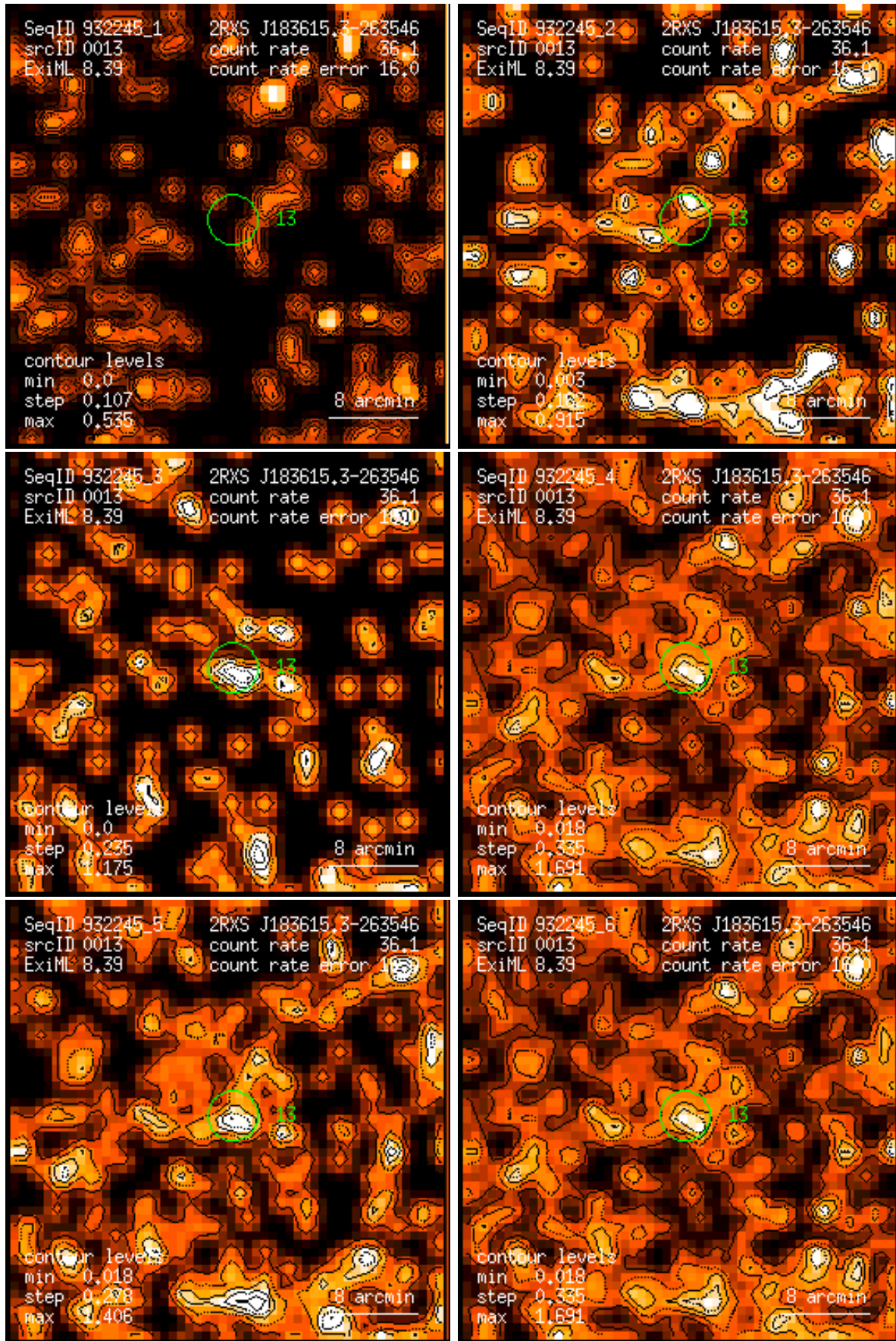
Figure 13: RASS 932245: detection 0013: band rate images, Gaussian filter: (1) PSPC channels 11 – 41, (2) 52 – 90, (3) 91 – 201, (4) 11 – 235, (5) 52 – 201, (6) 11 – 201. Broad band rates in counts/ks. Band rate contour levels in counts/ks/arcmin 2 .
