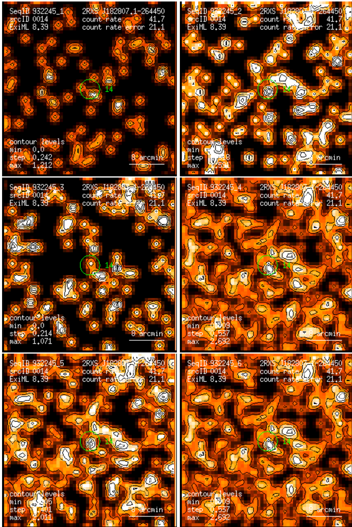
Figure 14: RASS 932245: detection 0014: band rate images, Gaussian filter: (1) PSPC channels 11 – 41, (2) 52 – 90, (3) 91 – 201, (4) 11 – 235, (5) 52 – 201, (6) 11 – 201. Broad band rates in counts/ks. Band rate contour levels in counts/ks/arcmin 2 .
