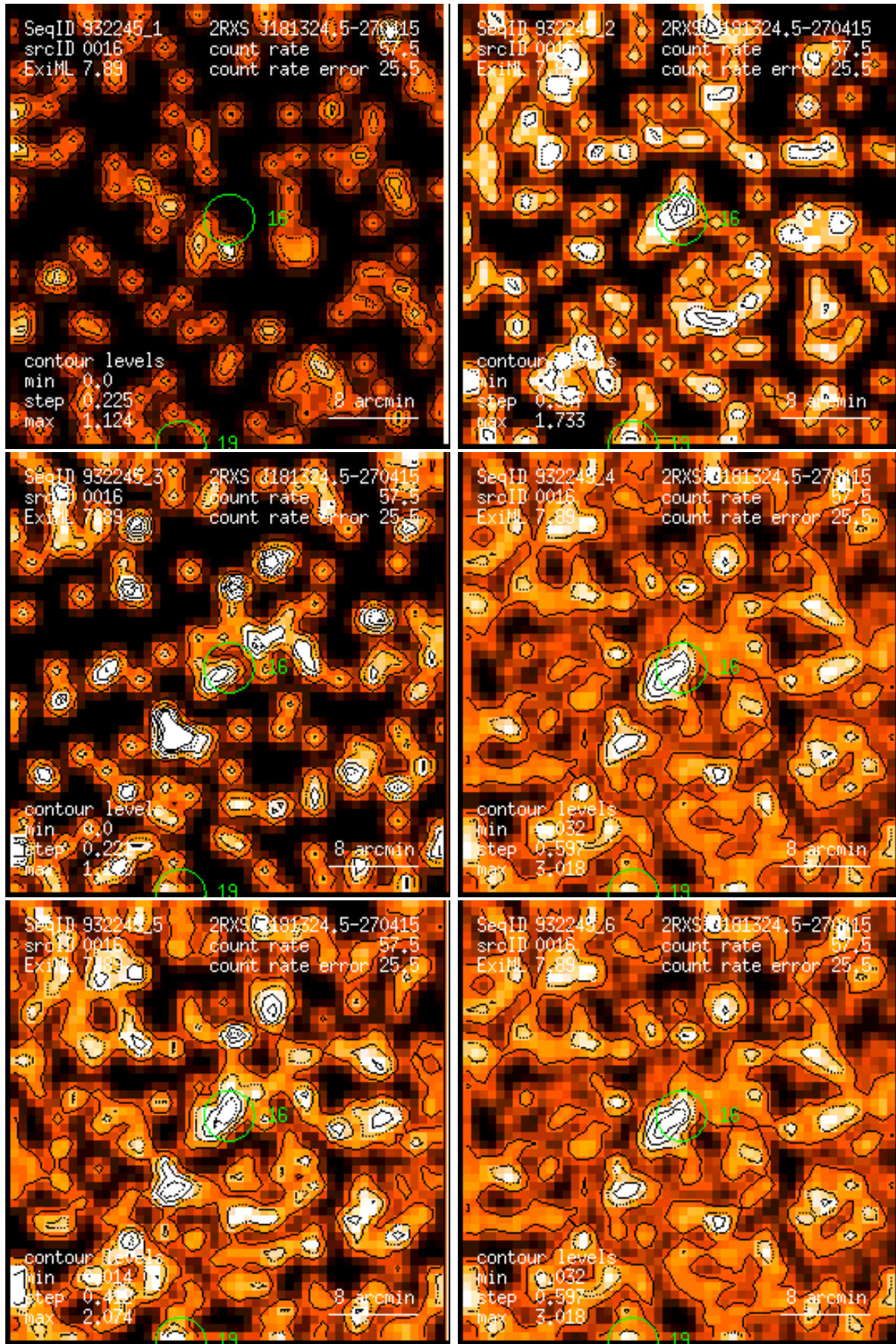
Figure 16: RASS 932245: detection 0016: band rate images, Gaussian filter: (1) PSPC channels 11 – 41, (2) 52 – 90, (3) 91 – 201, (4) 11 – 235, (5) 52 – 201, (6) 11 – 201. Broad band rates in counts/ks. Band rate contour levels in counts/ks/arcmin 2 .
