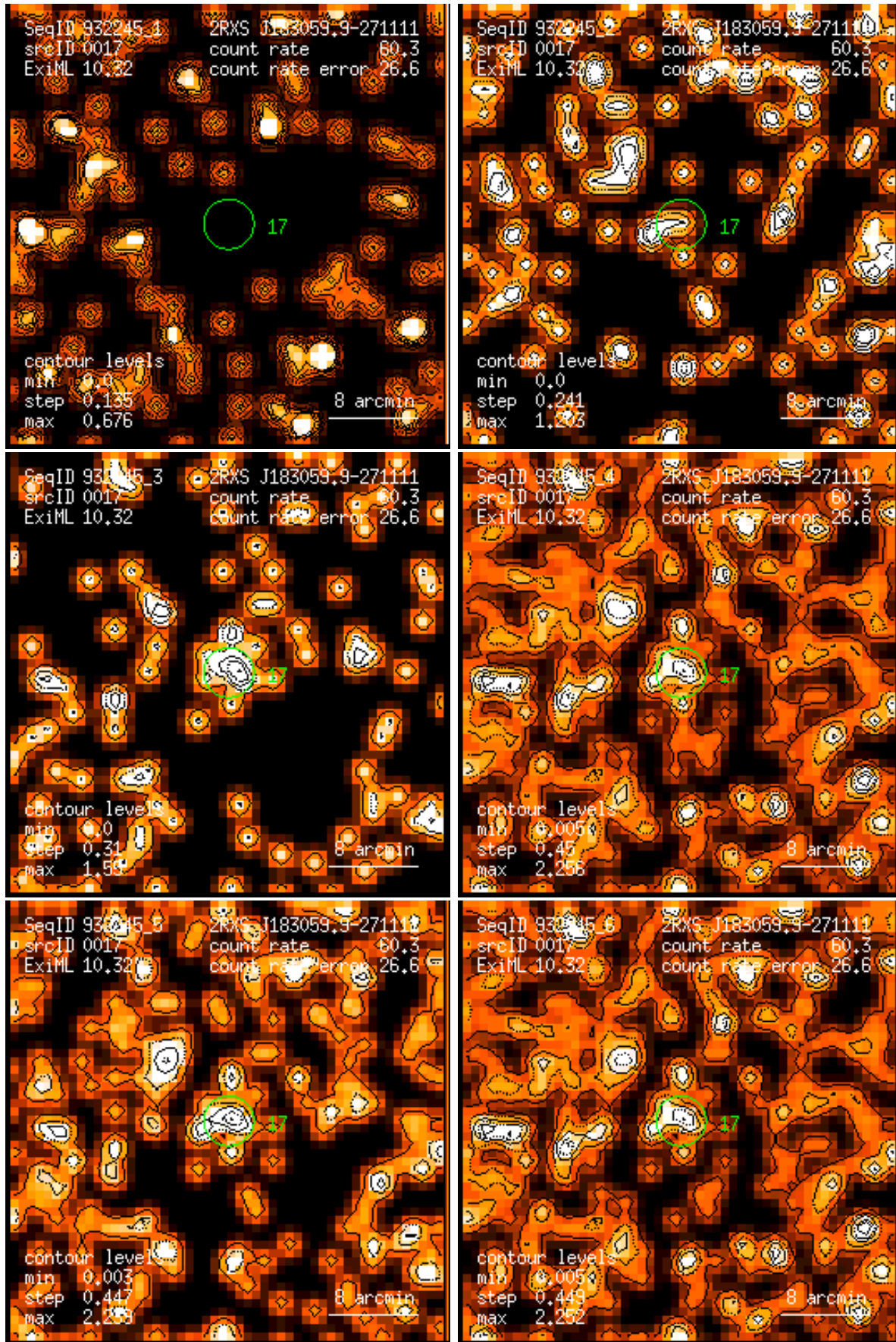
Figure 17: RASS 932245: detection 0017: band rate images, Gaussian filter: (1) PSPC channels 11 – 41, (2) 52 – 90, (3) 91 – 201, (4) 11 – 235, (5) 52 – 201, (6) 11 – 201. Broad band rates in counts/ks. Band rate contour levels in counts/ks/arcmin 2 .
