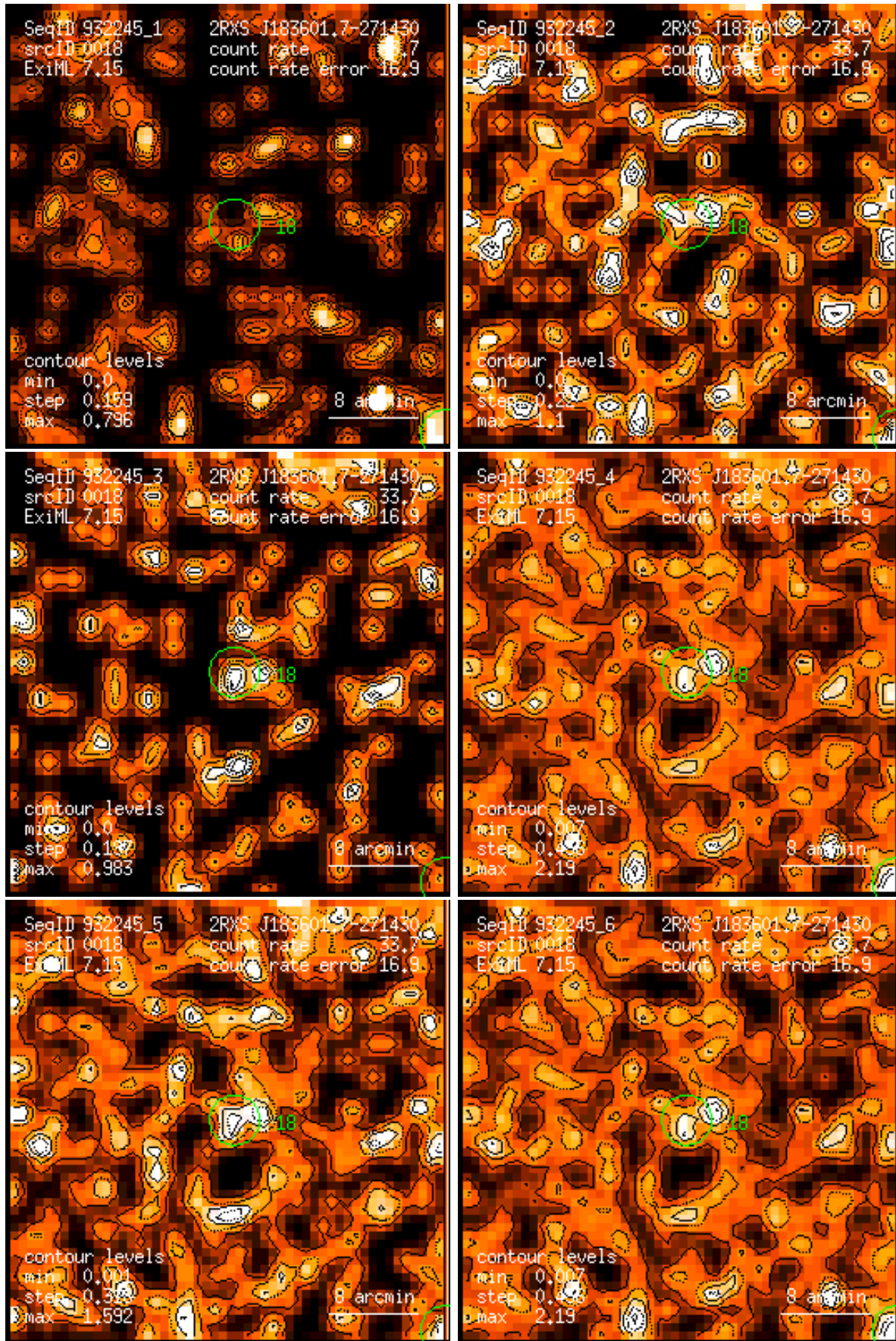
Figure 18: RASS 932245: detection 0018: band rate images, Gaussian filter: (1) PSPC channels 11 – 41, (2) 52 – 90, (3) 91 – 201, (4) 11 – 235, (5) 52 – 201, (6) 11 – 201. Broad band rates in counts/ks. Band rate contour levels in counts/ks/arcmin 2 .
