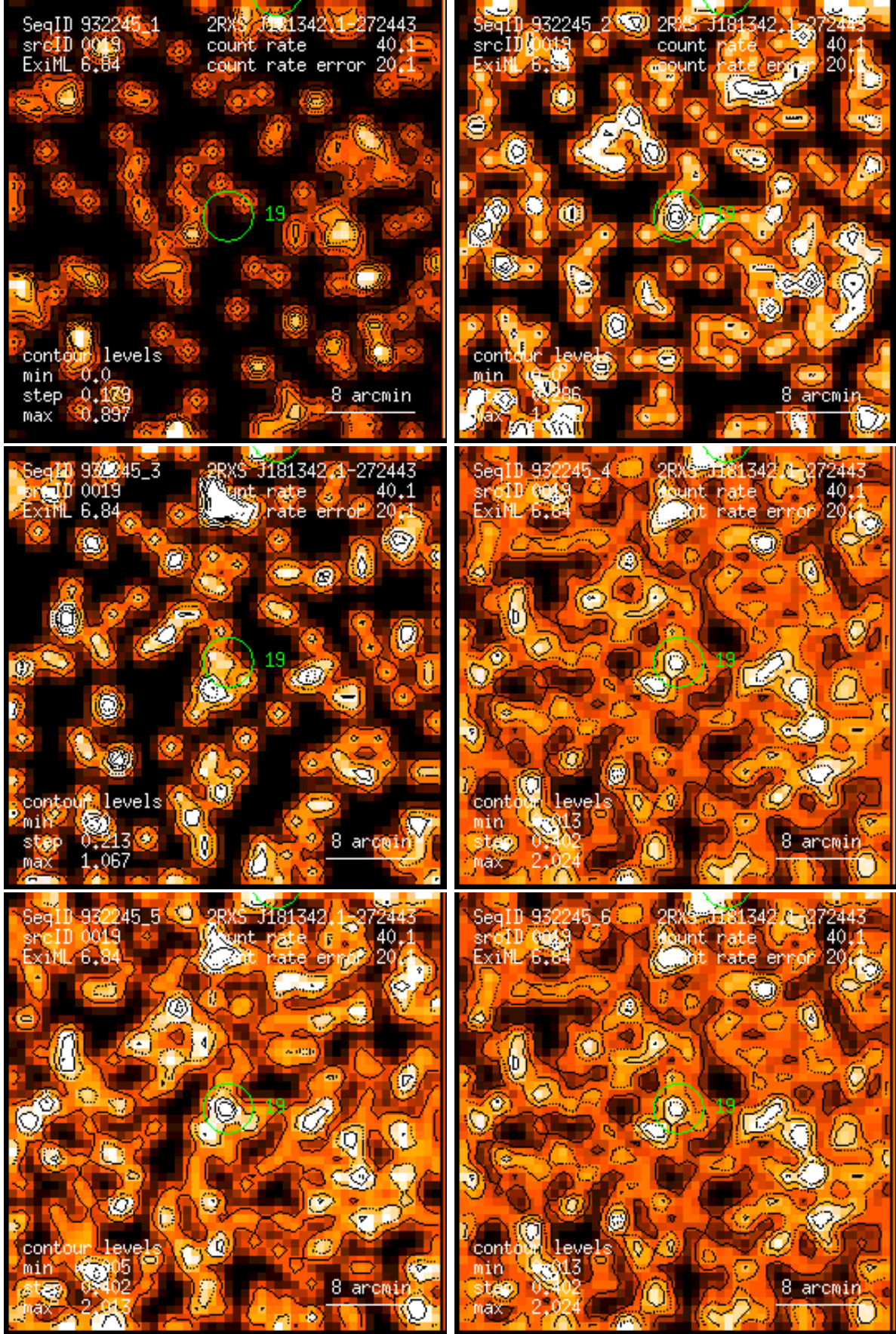
Figure 19: RASS 932245: detection 0019: band rate images, Gaussian filter: (1) PSPC channels 11 – 41, (2) 52 – 90, (3) 91 – 201, (4) 11 – 235, (5) 52 – 201, (6) 11 – 201. Broad band rates in counts/ks. Band rate contour levels in counts/ks/arcmin 2 .
