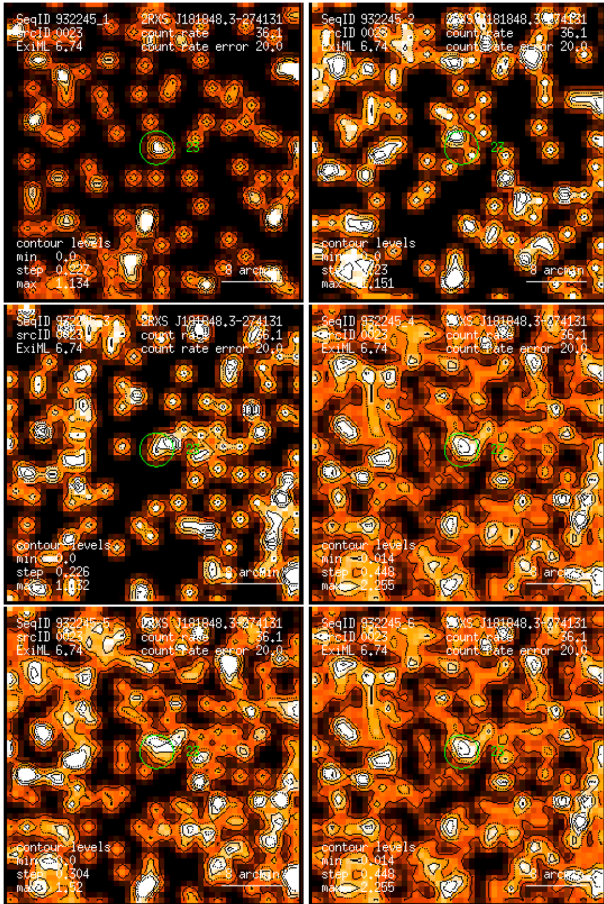
Figure 23: RASS 932245: detection 0023: band rate images, Gaussian filter: (1) PSPC channels 11 – 41, (2) 52 – 90, (3) 91 – 201, (4) 11 – 235, (5) 52 – 201, (6) 11 – 201. Broad band rates in counts/ks. Band rate contour levels in counts/ks/arcmin 2 .
