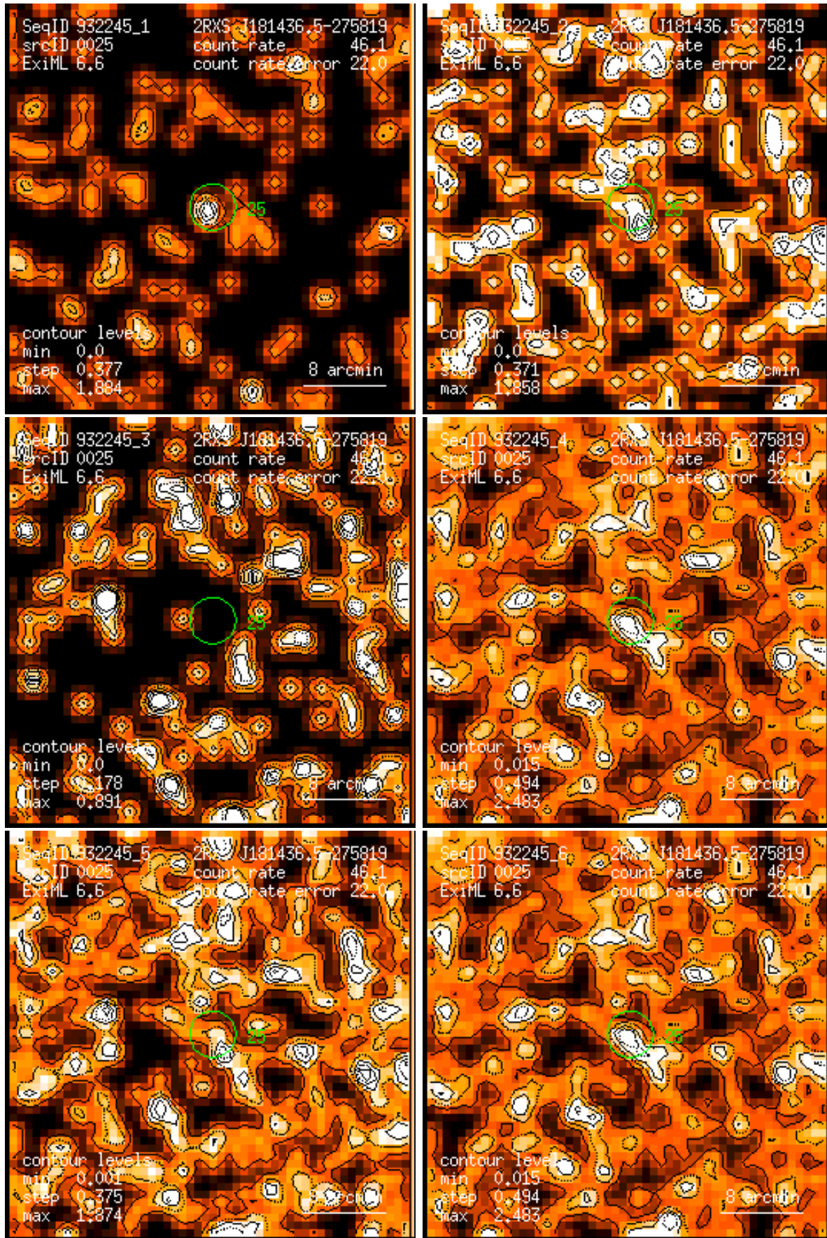
Figure 25: RASS 932245: detection 0025: band rate images, Gaussian filter: (1) PSPC channels 11 – 41, (2) 52 – 90, (3) 91 – 201, (4) 11 – 235, (5) 52 – 201, (6) 11 – 201. Broad band rates in counts/ks. Band rate contour levels in counts/ks/arcmin 2 .
