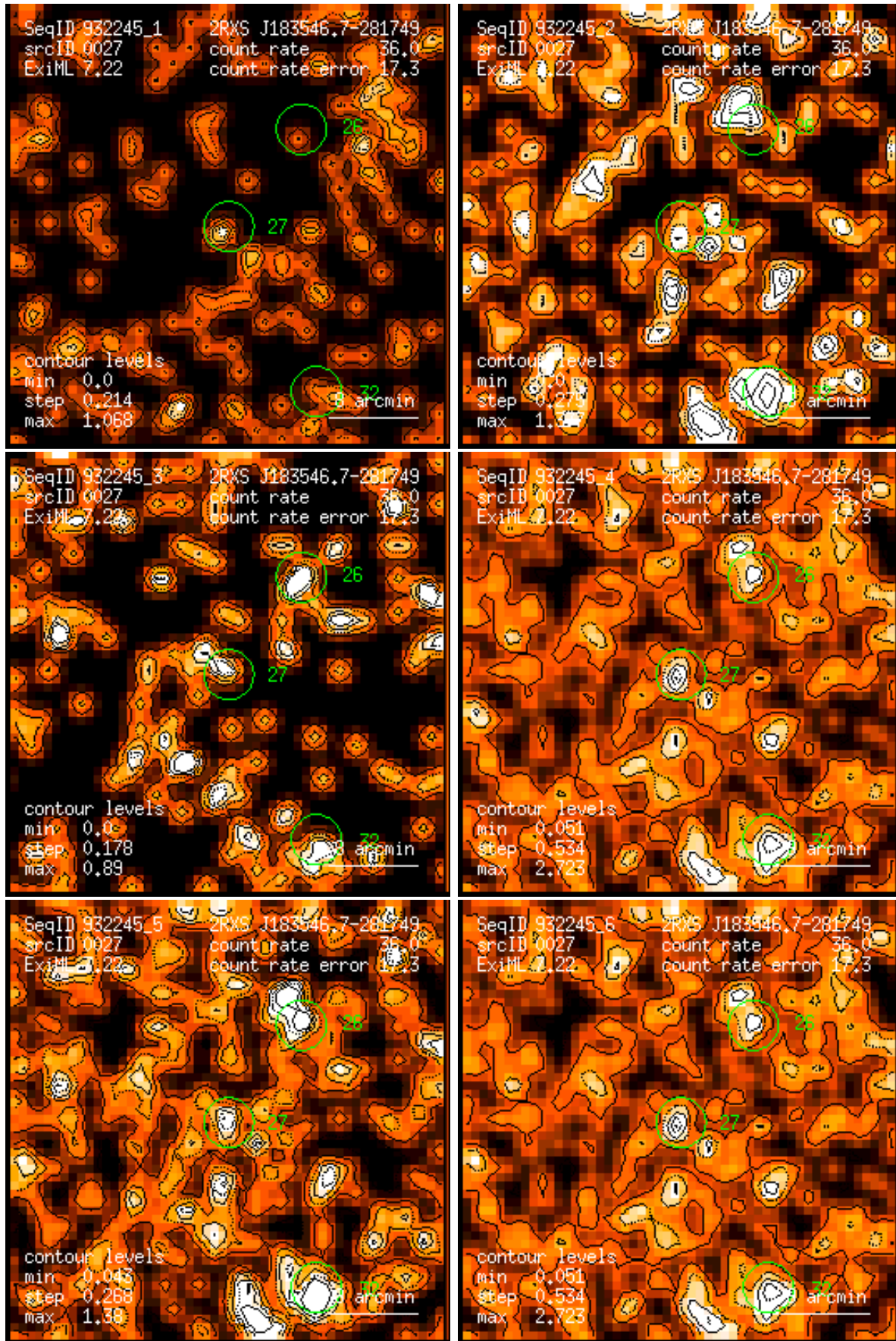
Figure 27: RASS 932245: detection 0027: band rate images, Gaussian filter: (1) PSPC channels 11 – 41, (2) 52 – 90, (3) 91 – 201, (4) 11 – 235, (5) 52 – 201, (6) 11 – 201. Broad band rates in counts/ks. Band rate contour levels in counts/ks/arcmin 2 .
