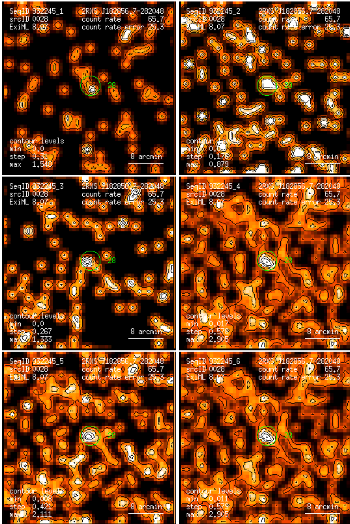
Figure 28: RASS 932245: detection 0028: band rate images, Gaussian filter: (1) PSPC channels 11 – 41, (2) 52 – 90, (3) 91 – 201, (4) 11 – 235, (5) 52 – 201, (6) 11 – 201. Broad band rates in counts/ks. Band rate contour levels in counts/ks/arcmin 2 .
