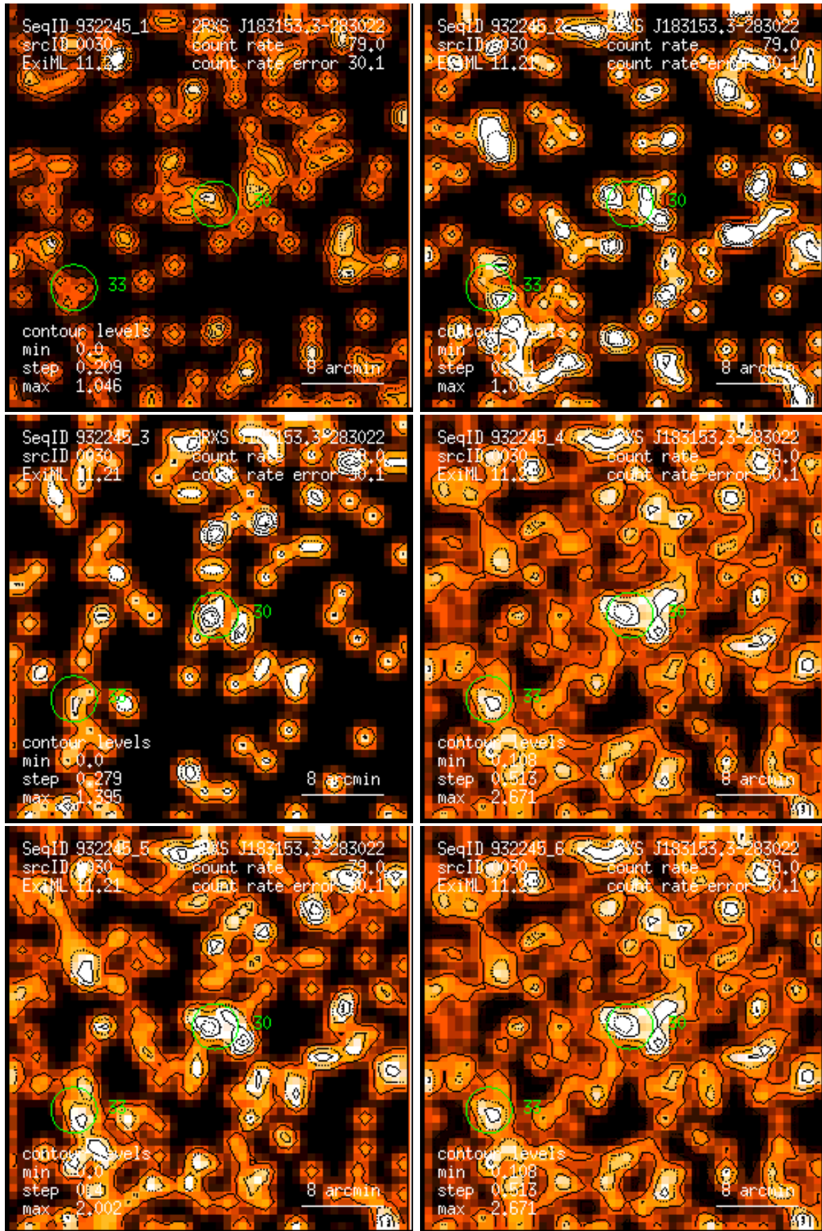
Figure 30: RASS 932245: detection 0030: band rate images, Gaussian filter: (1) PSPC channels 11 – 41, (2) 52 – 90, (3) 91 – 201, (4) 11 – 235, (5) 52 – 201, (6) 11 – 201. Broad band rates in counts/ks. Band rate contour levels in counts/ks/arcmin 2 .
