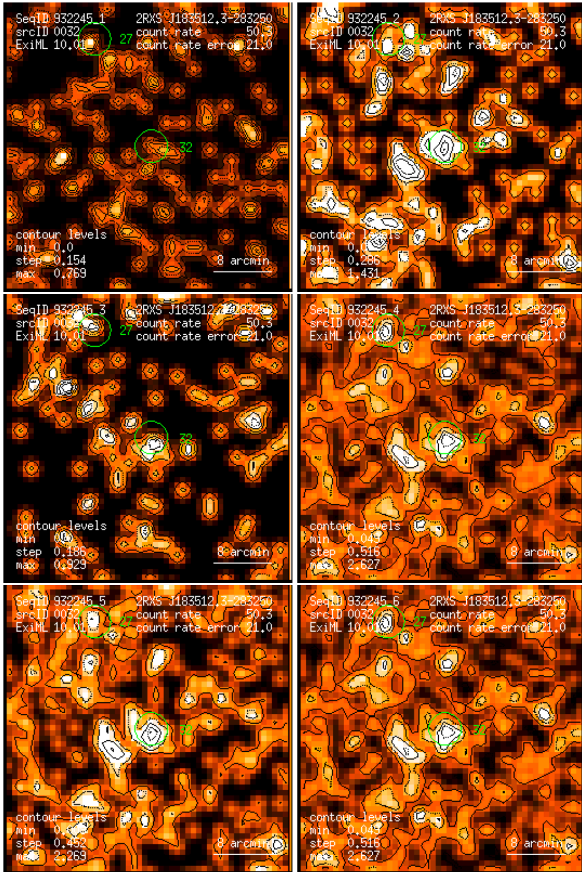
Figure 32: RASS 932245: detection 0032: band rate images, Gaussian filter: (1) PSPC channels 11 – 41, (2) 52 – 90, (3) 91 – 201, (4) 11 – 235, (5) 52 – 201, (6) 11 – 201. Broad band rates in counts/ks. Band rate contour levels in counts/ks/arcmin 2 .
