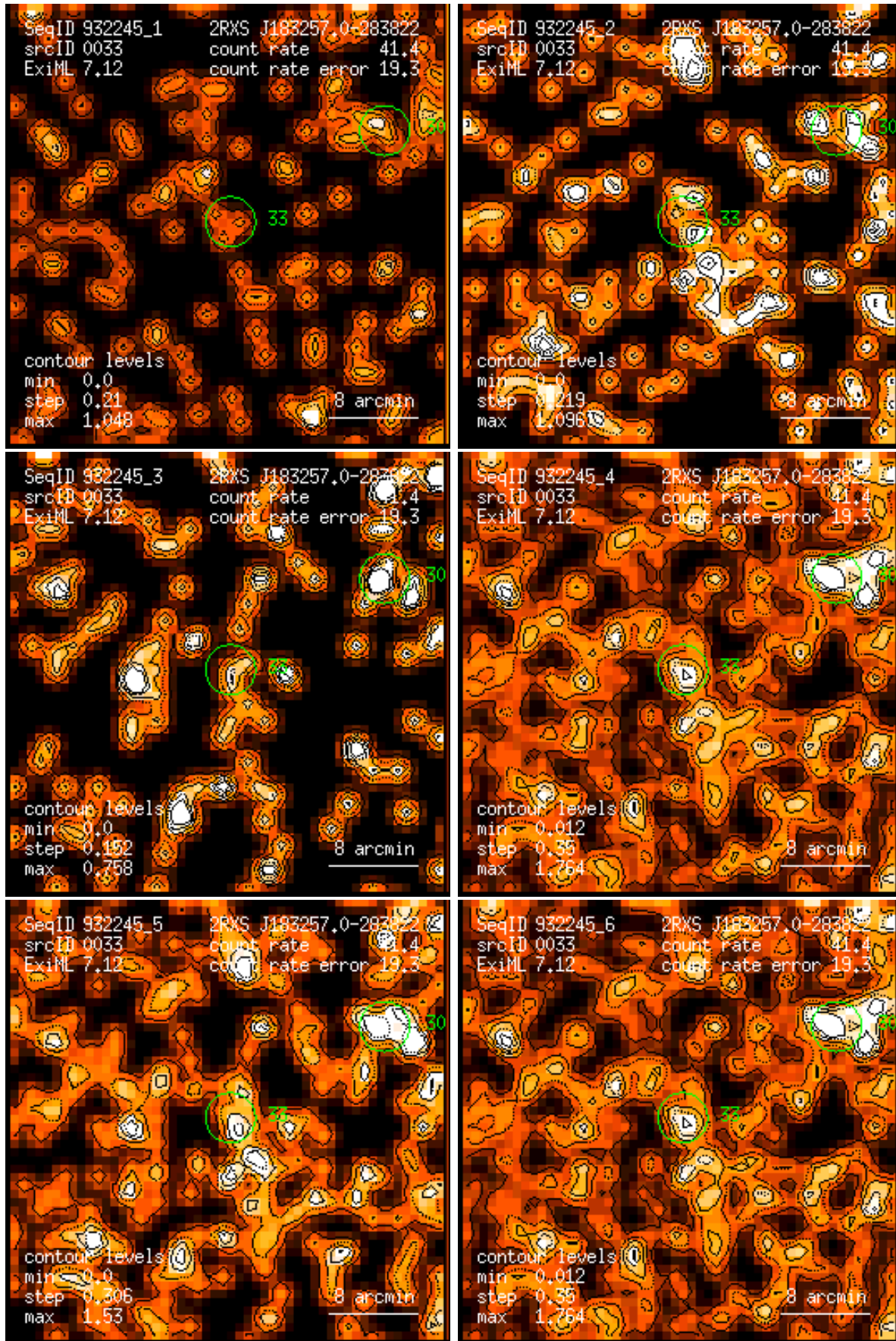
Figure 33: RASS 932245: detection 0033: band rate images, Gaussian filter: (1) PSPC channels 11 – 41, (2) 52 – 90, (3) 91 – 201, (4) 11 – 235, (5) 52 – 201, (6) 11 – 201. Broad band rates in counts/ks. Band rate contour levels in counts/ks/arcmin 2 .
