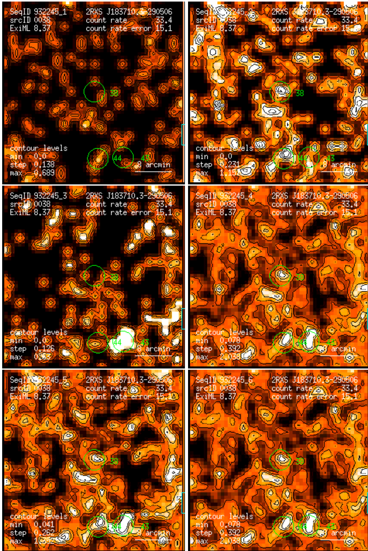
Figure 38: RASS 932245: detection 0038: band rate images, Gaussian filter: (1) PSPC channels 11 – 41, (2) 52 – 90, (3) 91 – 201, (4) 11 – 235, (5) 52 – 201, (6) 11 – 201. Broad band rates in counts/ks. Band rate contour levels in counts/ks/arcmin 2 .
