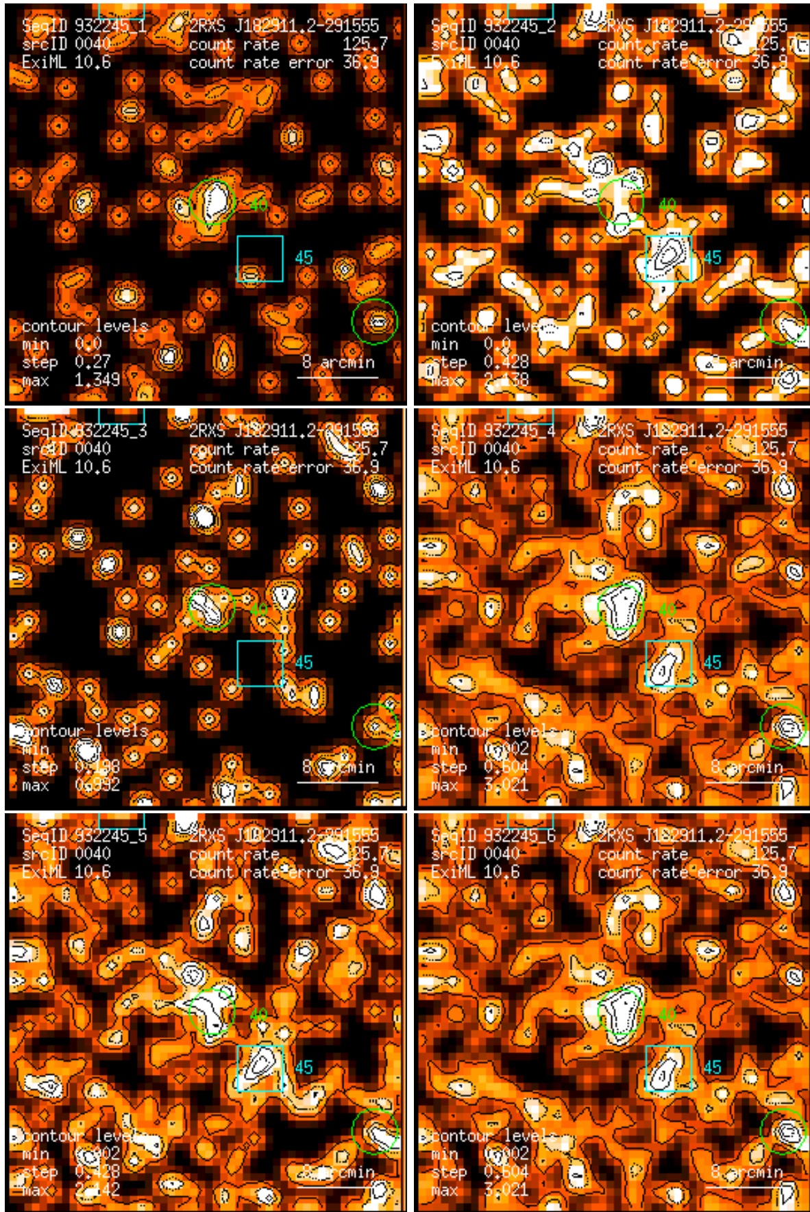
Figure 40: RASS 932245: detection 0040: band rate images, Gaussian filter: (1) PSPC channels 11 – 41, (2) 52 – 90, (3) 91 – 201, (4) 11 – 235, (5) 52 – 201, (6) 11 – 201. Broad band rates in counts/ks. Band rate contour levels in counts/ks/arcmin 2 .
