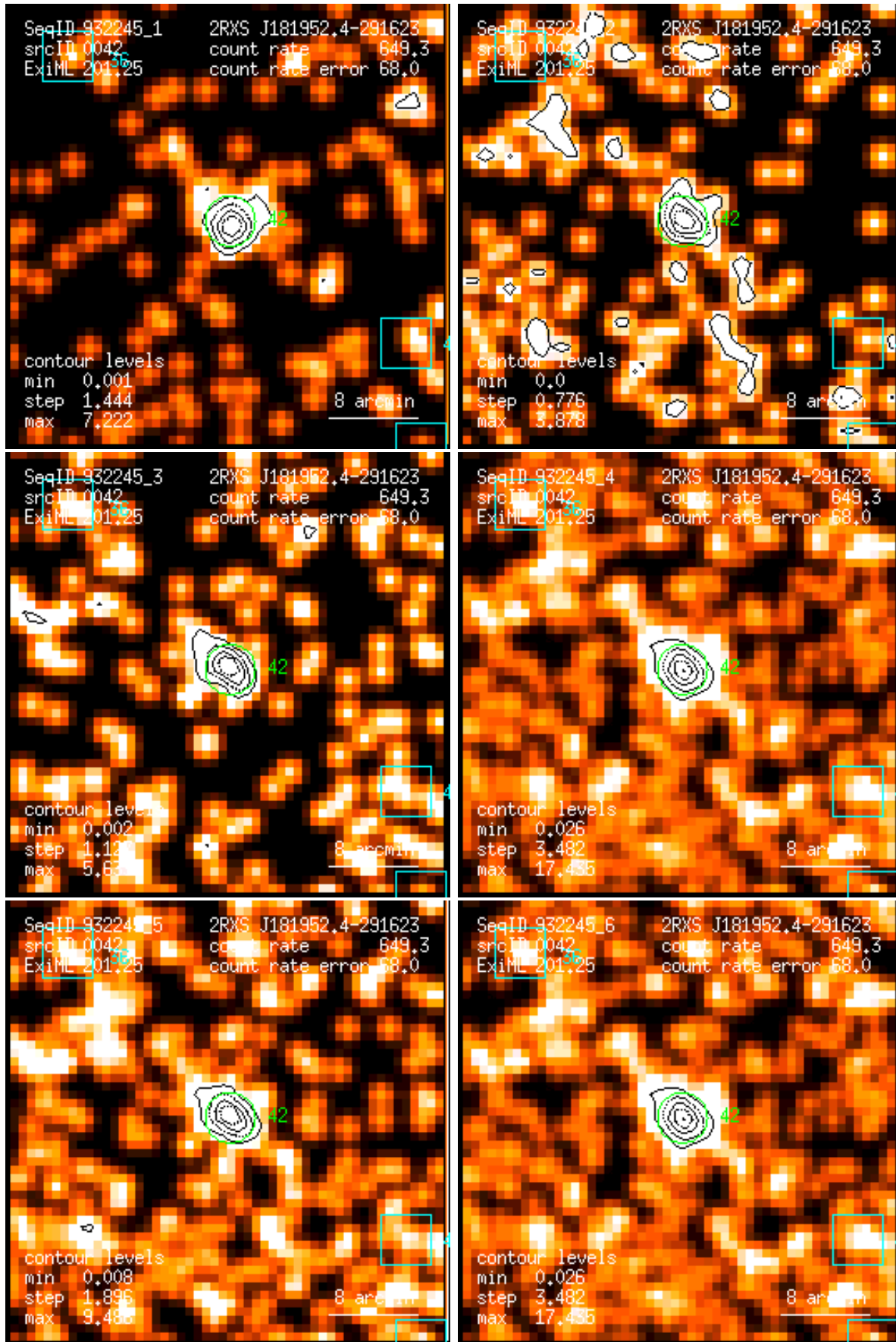
Figure 42: RASS 932245: detection 0042: band rate images, Gaussian filter: (1) PSPC channels 11 – 41, (2) 52 – 90, (3) 91 – 201, (4) 11 – 235, (5) 52 – 201, (6) 11 – 201. Broad band rates in counts/ks. Band rate contour levels in counts/ks/arcmin 2 .
