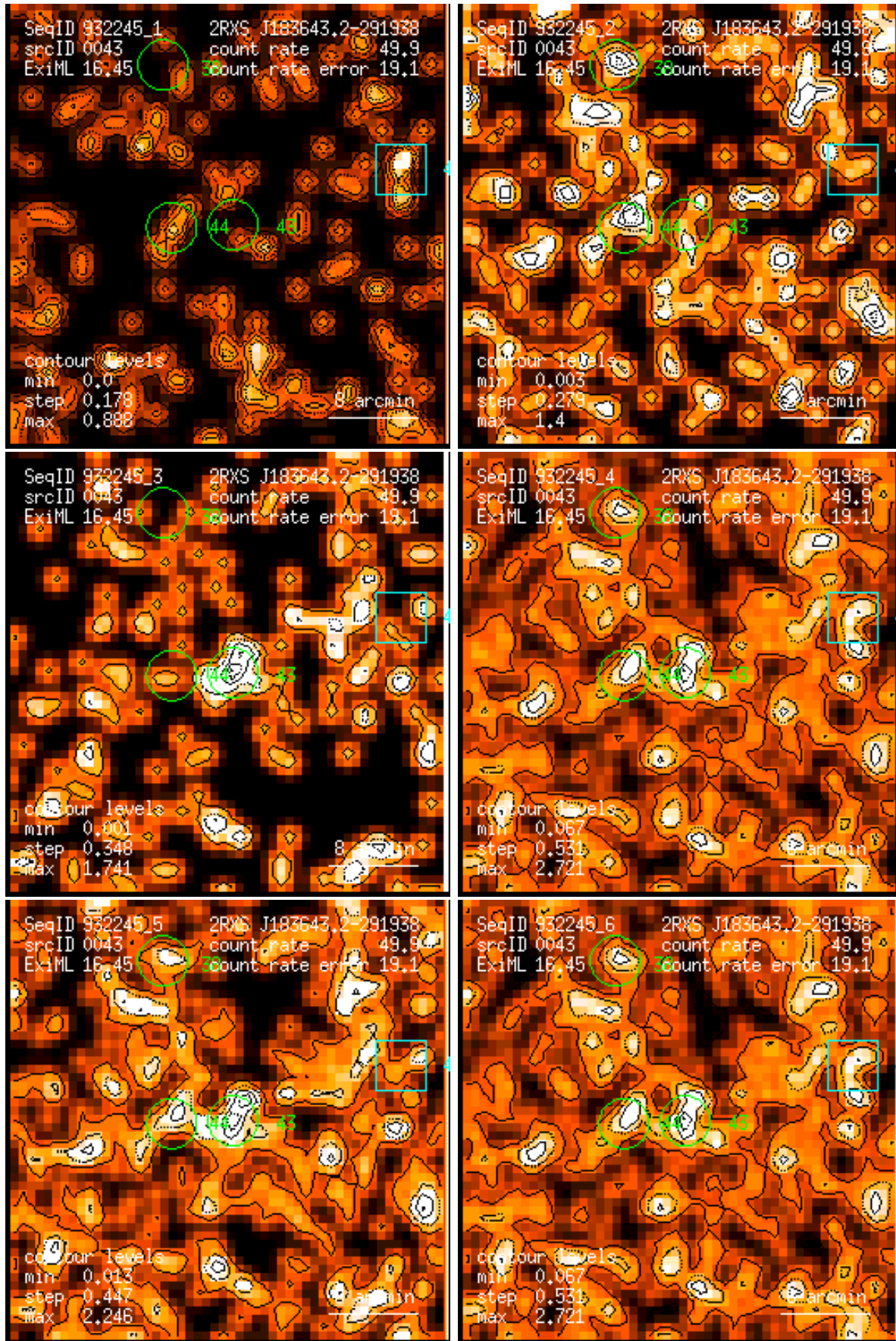
Figure 43: RASS 932245: detection 0043: band rate images, Gaussian filter: (1) PSPC channels 11 – 41, (2) 52 – 90, (3) 91 – 201, (4) 11 – 235, (5) 52 – 201, (6) 11 – 201. Broad band rates in counts/ks. Band rate contour levels in counts/ks/arcmin 2 .
