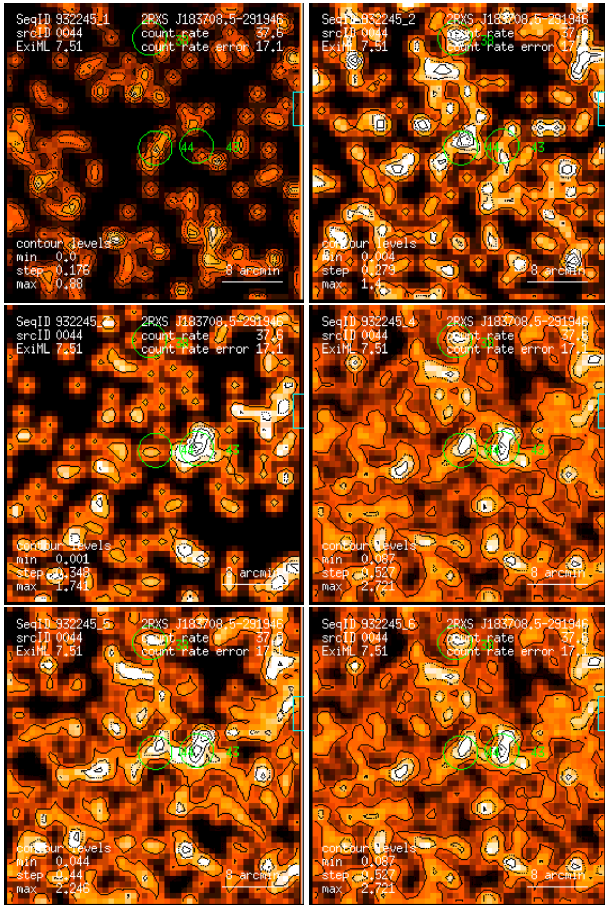
Figure 44: RASS 932245: detection 0044: band rate images, Gaussian filter: (1) PSPC channels 11 – 41, (2) 52 – 90, (3) 91 – 201, (4) 11 – 235, (5) 52 – 201, (6) 11 – 201. Broad band rates in counts/ks. Band rate contour levels in counts/ks/arcmin 2 .
