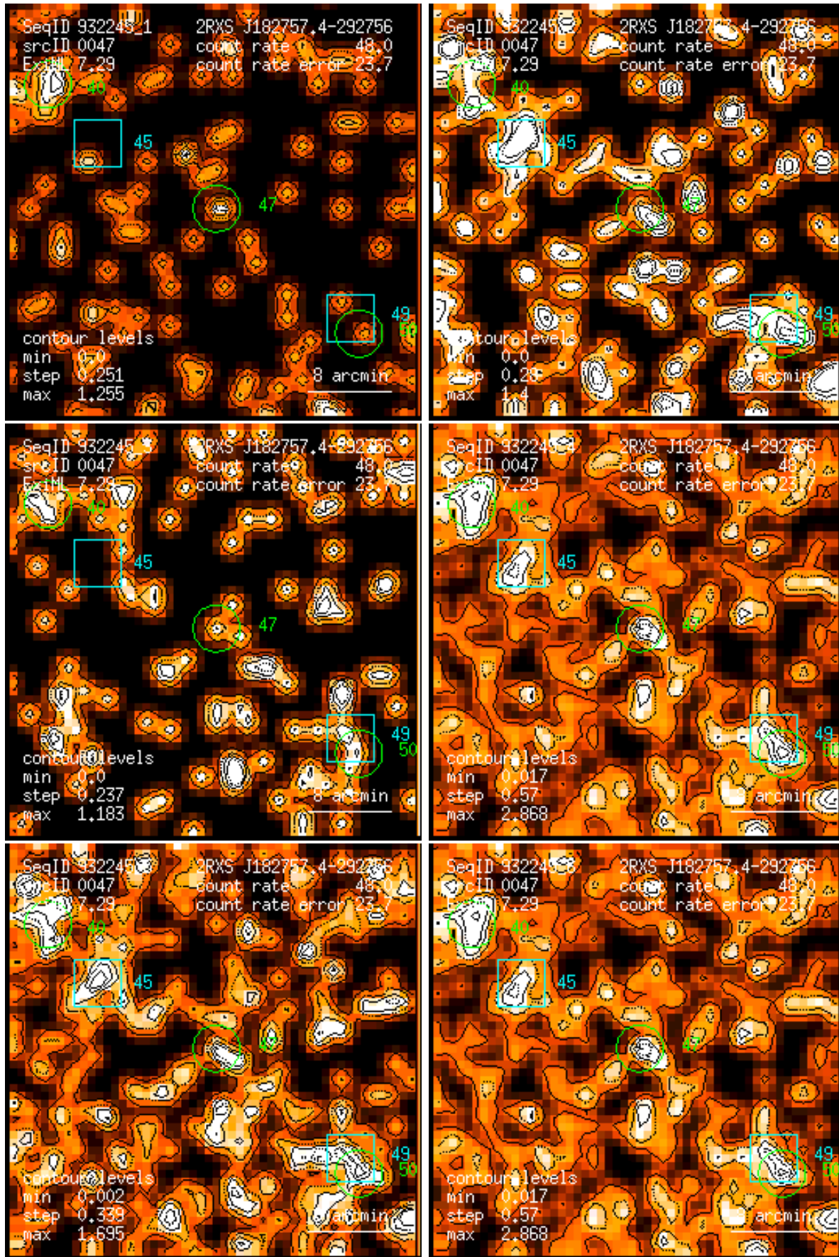
Figure 47: RASS 932245: detection 0047: band rate images, Gaussian filter: (1) PSPC channels 11 – 41, (2) 52 – 90, (3) 91 – 201, (4) 11 – 235, (5) 52 – 201, (6) 11 – 201. Broad band rates in counts/ks. Band rate contour levels in counts/ks/arcmin 2 .
